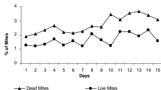
Figure 1. Daily mean percentage of live and dead mites collected in five Africanized bee colonies.
