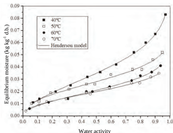
Figure 2. Sorption isotherm of grapefruit seeds at different temperatures.
