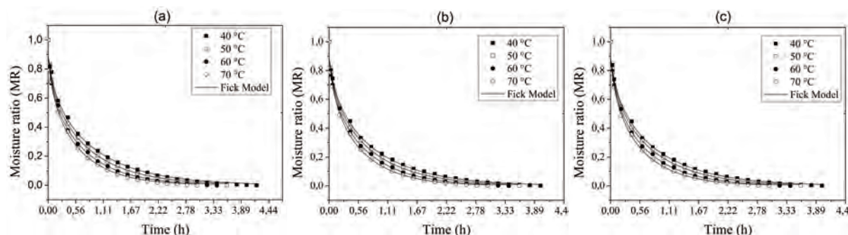
Figure 3. Drying curves: (a) 0.6 \text{ m s}^{-1} ; (b) 1.0 \text{ m s}^{-1} ; (c) 1.4 \text{ m s}^{-1} .
