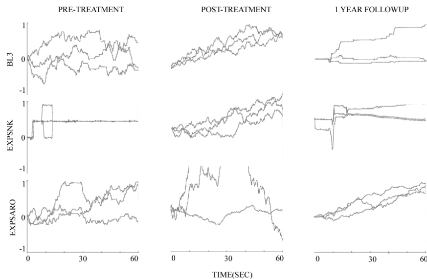
FIGURE 2. Phase synchronization between channels P3-P4, T3-T4, and T5-T6 during baseline (upper row), exposure to snake pictures (middle row), and exposure to equivalent arousal pictures (lower row) at pre-treatment (left column), post-treatment (middle column) and one-year follow-up (right column).
