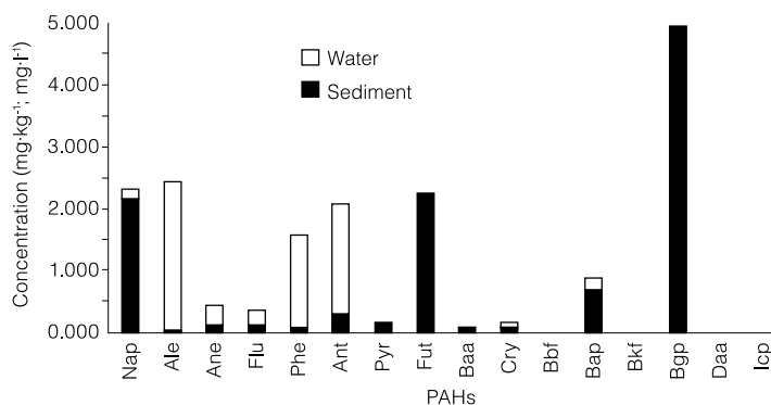
Figure 2. Total concentration of 16 priority polycyclic aromatic hydrocarbons in water and sediment; Nap: naphthalene, Ale: acenaphthylene, Ane: acenaphthene, Flu: fluorene, Phe: phenanthrene, Ant: anthracene, Pyr: pyrene, Fut: fluoranthene, Baa: benzo[a]anthracene, Cry: chrysene, Bbf: benzo[b]fluoranthene, Bap: benzo[a]pyrene, Bkf: benzo[k]fluoranthene, Bgp: benzo[g,h,i]perylene, Daa: dibenzo[a,h]anthracene, Icp: indeno[1,2,3-cd]pyrene (concentrations of Bbf, Bkf, Daa, and Icp were below minimum level of detection).
