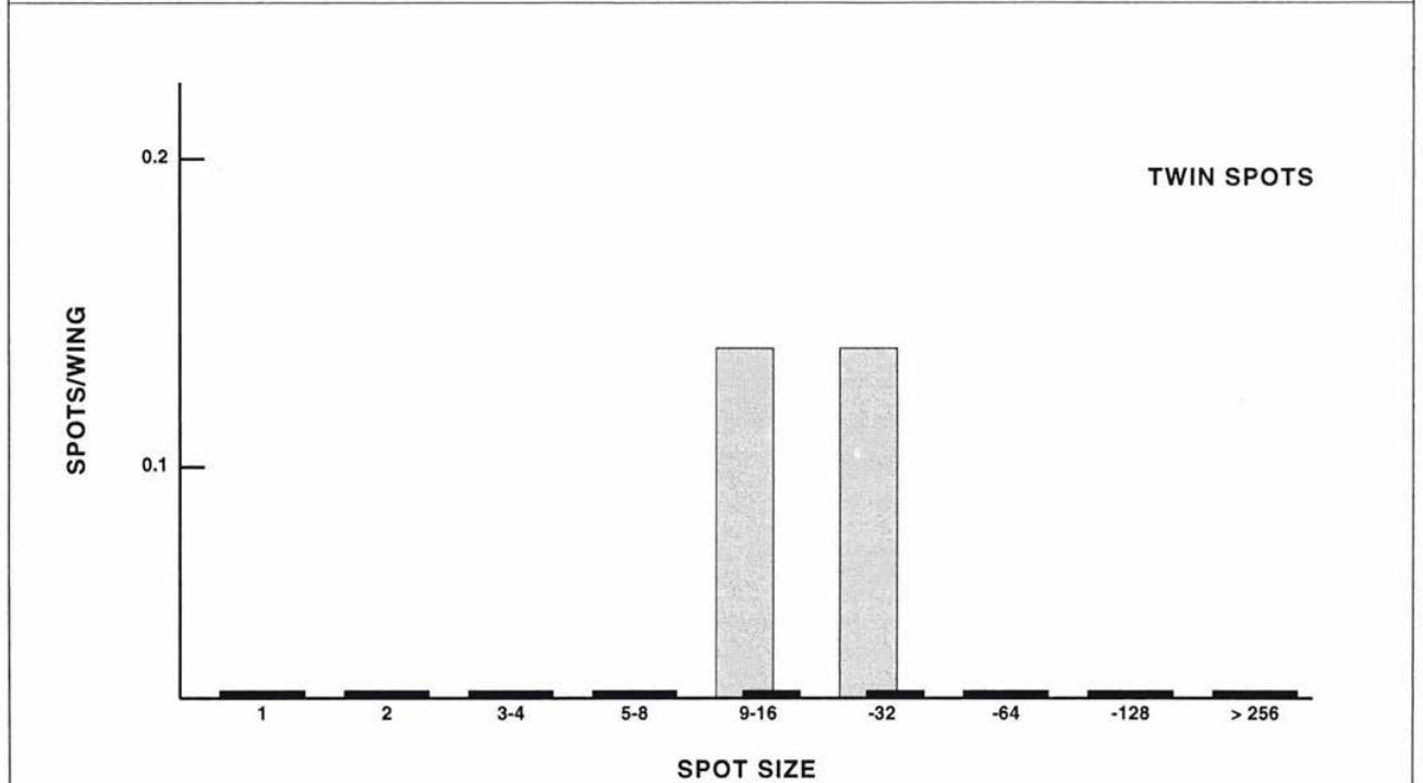
Fig. 2. Spot frequencies in 80 wings, shown as size class distributions, induced in 72 h larvae by 300 mM of saccharin , control
