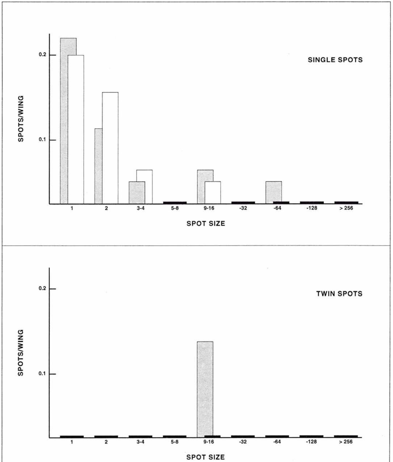
Fig. 1. Spot frequencies in 80 wings, shown as size class distributions, induced in 48 h larvae by 300 mM of saccharin , control
