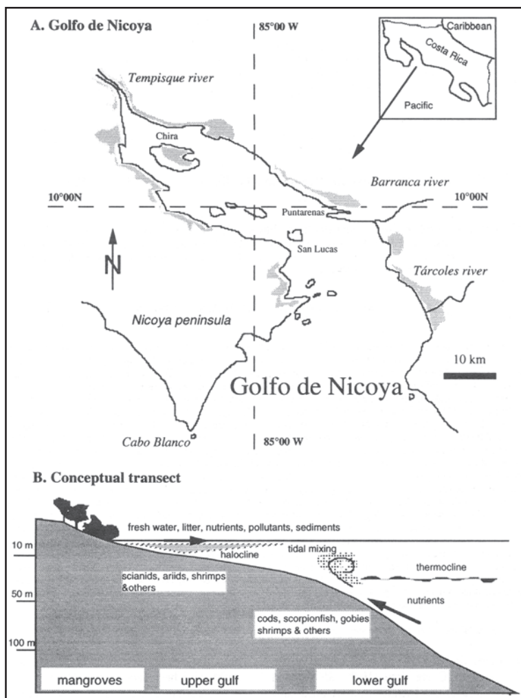
Fig. 1. Gulf of Nicoya, Costa Rica. A. Study area; B. Conceptual transect. Reprinted from Wolff, M., J. Chavarría, V. Koch and J. A. Vargas. 1998. A trophic flow model of the Golfo de Nicoya, Costa Rica. Rev. Biol. Trop. 46 (Supl. 6): 63-79, with permission from RBT.
