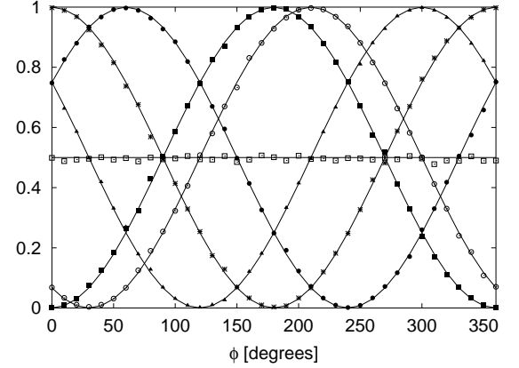
FIG. 3: Simulation results for the DLM-network shown in Fig. 1. Input channel 0 receives (\cos \psi_0, \sin \psi_0) with probability one. A uniform random number in the range [0, 360] is used to choose the angle \psi_0 . Input channel 1 receives no events. Each data point represents 10000 events ( N_0 + N_1 = N_2 + N_3 = 10000 ). Initially the rotation angle \phi_0 = 0 and after each set of 10000 events, \phi_0 is increased by 10^\circ . Markers give the simulation results for the normalized intensities as a function of \phi = \phi_0 - \phi_1 . Open squares: N_0/(N_0 + N_1) ; Solid squares: N_2/(N_2 + N_3) for \phi_1 = 0 ; Open circles: N_2/(N_2 + N_3) for \phi_1 = 30^\circ ; Bullets: N_2/(N_2 + N_3) for \phi_1 = 240^\circ ; Asterisks: N_3/(N_2 + N_3) for \phi_1 = 0 ; Solid triangles: N_3/(N_2 + N_3) for \phi_1 = 300^\circ . Lines represent the results of quantum theory [18].
