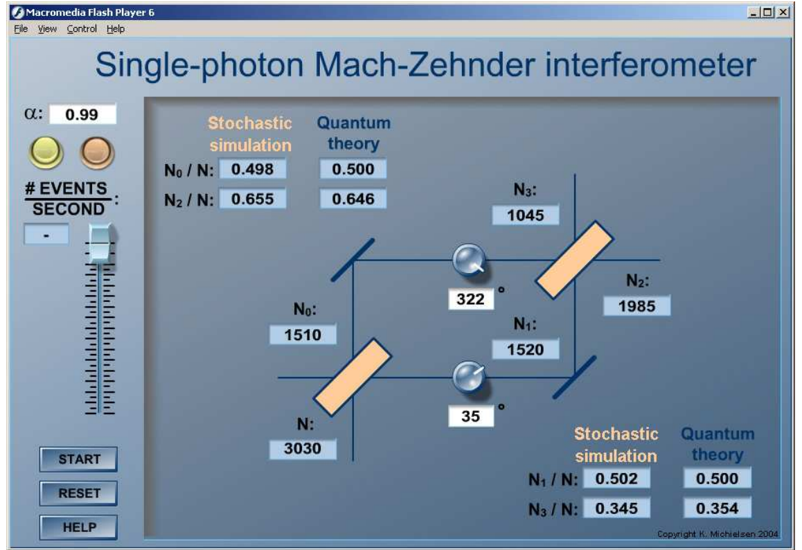
FIG. 1: (color online) Snapshot of an interactive event-by-event simulator of a Mach-Zehnder interferometer [16]. The main panel shows the layout of the interferometer. Particles emerge from a source (not shown) located at the bottom of the leftmost vertical line. After leaving the first beam splitter in either the vertical or horizontal direction, the particles experience time delays that are specified by the controls on the lines. In this example, the time delays correspond to the phase shifts \phi_0 = 35^\circ and \phi_1 = 322^\circ in the wave mechanical description. The thin, 45^\circ -tilted lines act as perfect mirrors. When a particle leaves the system at the top right, it adds to the count of either detector N_2 or N_3 . Additional detectors ( N_0 , N_1 ) count the number of particles on the corresponding lines. The other cells give the ratio of the detector counts to the total number of particles (messages) processed and also the corresponding probability of the quantum mechanical description. At any time, the user can choose between a strictly deterministic and a stochastic event-by-event simulation by pressing the buttons at the top of the control panel.
