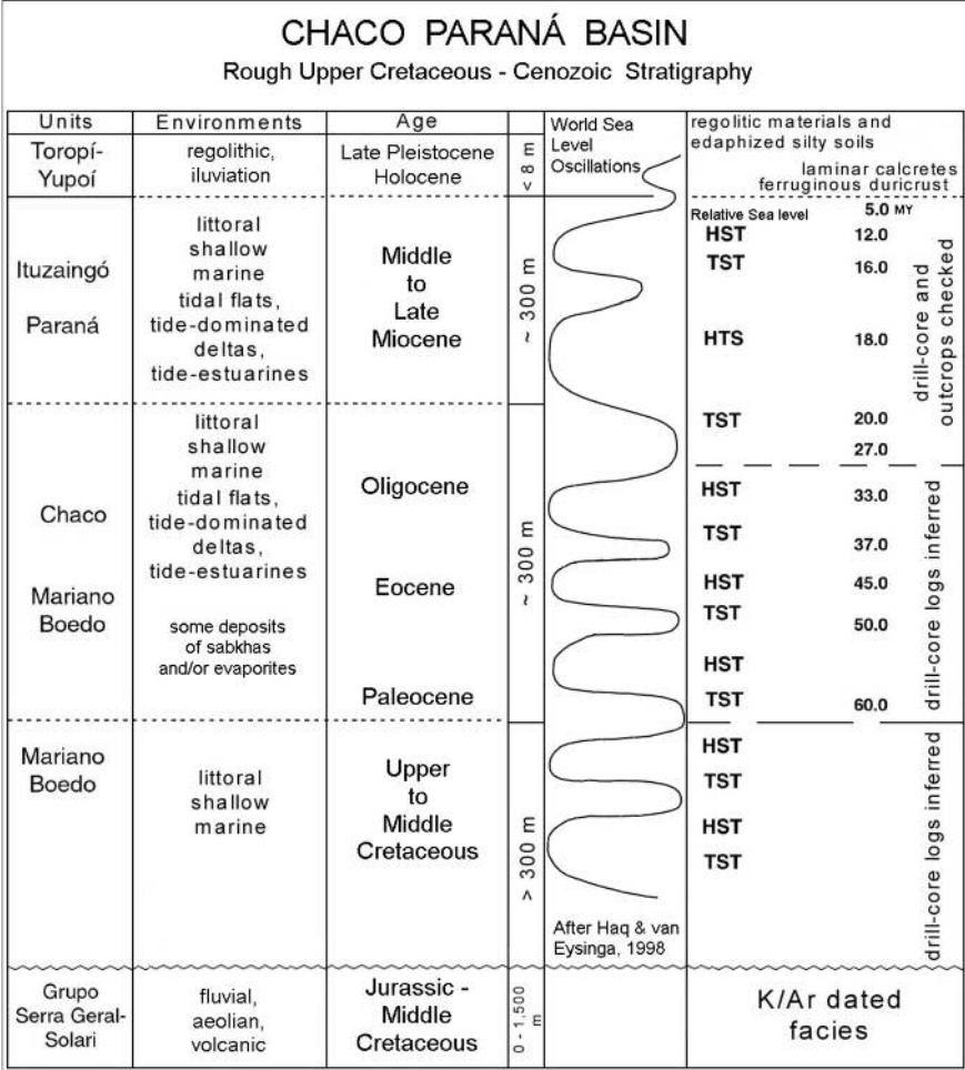
Figure 9. A sketch draw that shows rough Upper Cretaceous - Cenozoic Stratigraphy proposition related to the Chaco Paraná Basin regional rift system basin from the past 75 m.y.
