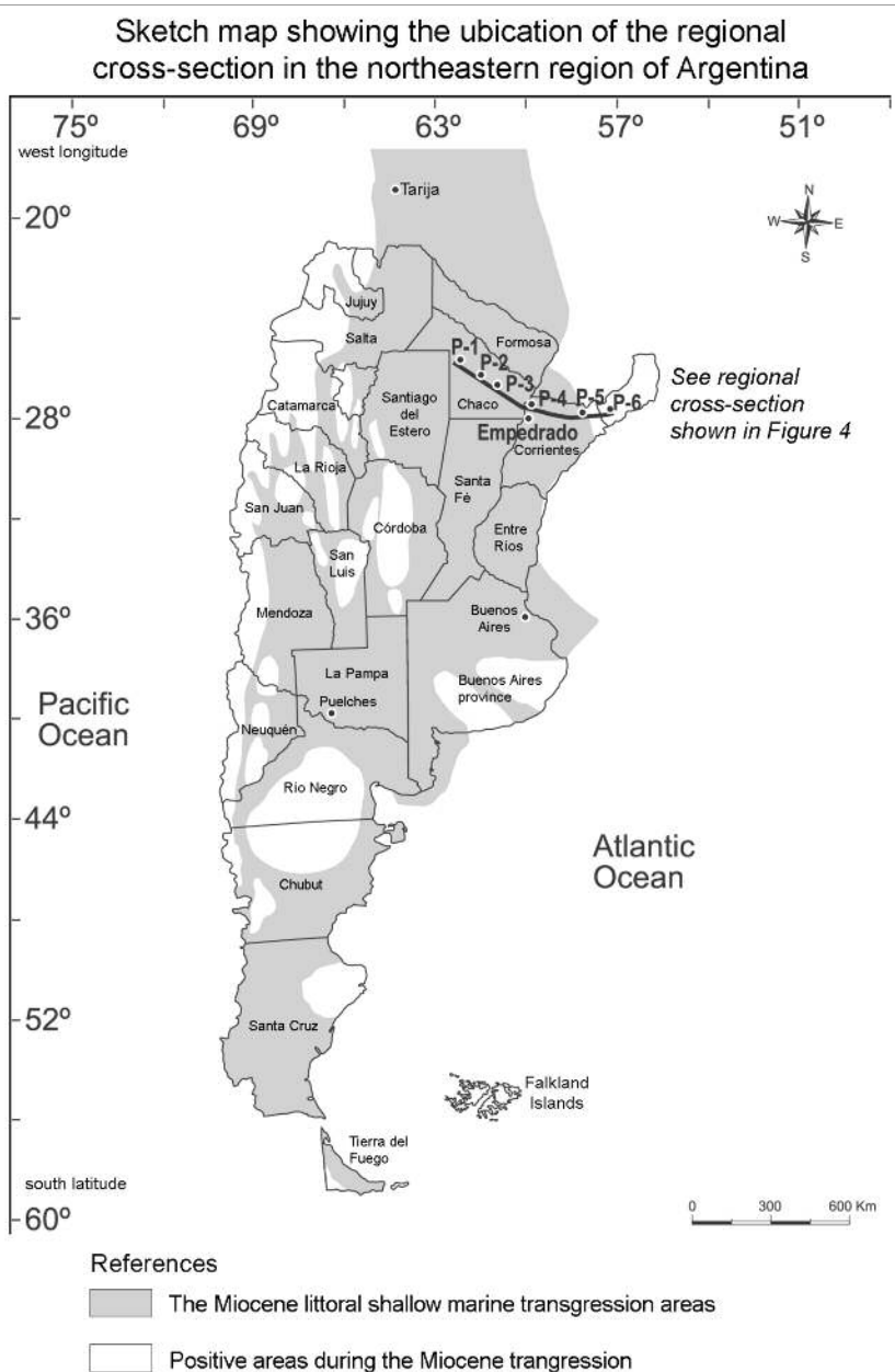
Figure 3. Sketch map that shows the ubication of the regional cross-section in the northeastern region of Argentina. Note the Puelches city location. The greyed zones correspond to the Miocene Sea transgression areas
