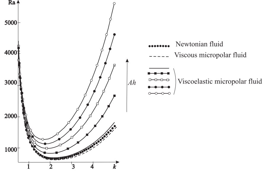
Figure 2: Neutral curves
