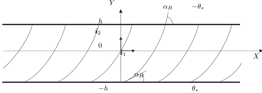
Figure 1: Plane layer of micropolar fluid
