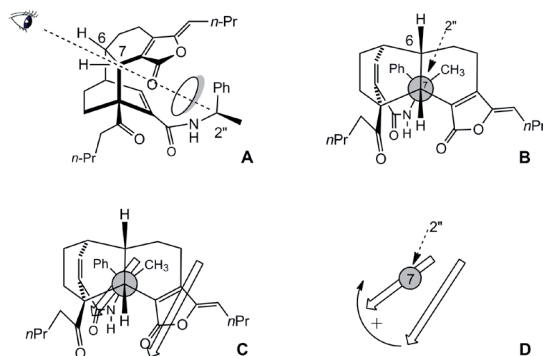
Fig. 4. A and B: Newman projections for (+)-7 between five \sigma bonds, with C–7 at the front and C–2'' at the rear. C and D: Spatial arrangement of the transition dipoles (arrows) for (+)-7.
