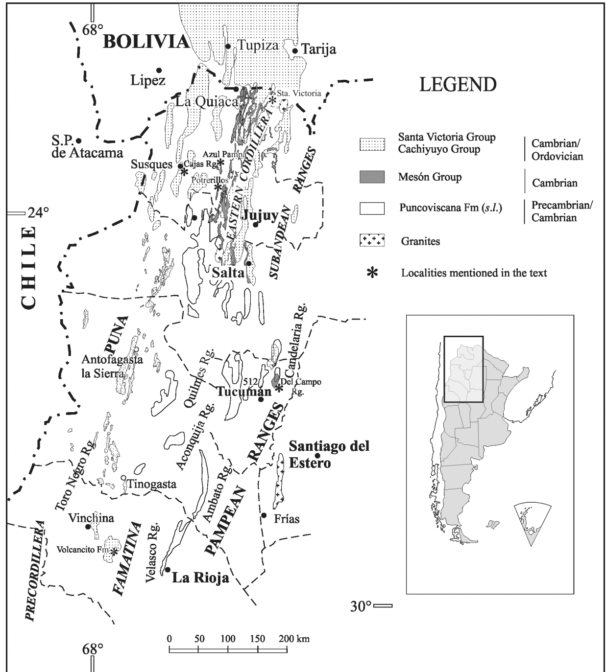
FIGURE 1 Location and distribution of Cambrian stratigraphic units (Precambrian-Cambrian Puncoviscana Formation ( s.l. ), the Cambrian Mesón Group and the Cambro-Ordovician Santa Victoria Group) in northwestern Argentina and location of significant outcrop zones mentioned in the text.
