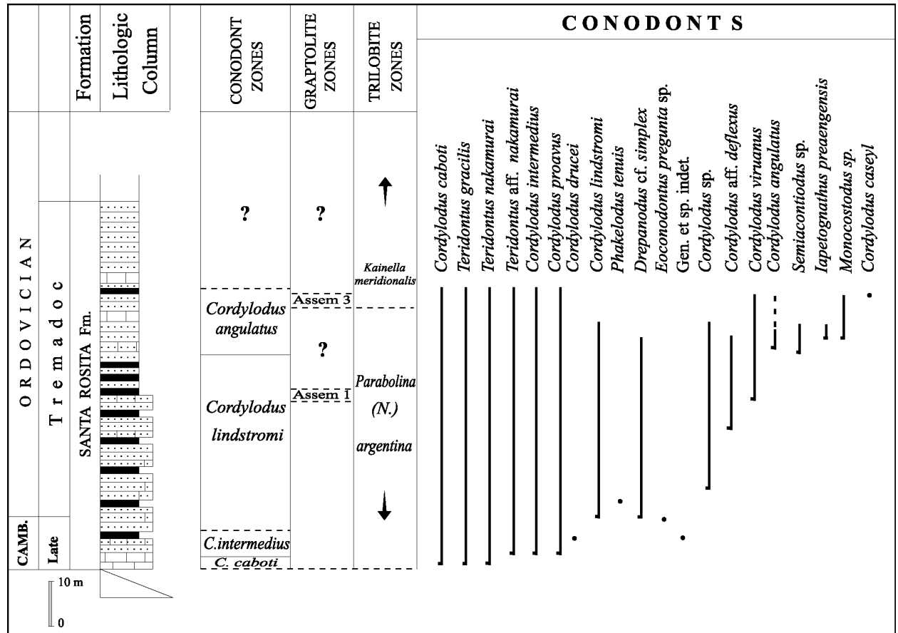
FIGURE 6 Stratigraphic sketch and biostratigraphic framework for the Cambro-Ordovician transition in the study area (lower part of Santa Victoria Group). The stratotype for the Cambrian-Ordovician boundary at the Sierra de Cajas is shown (based in Rao and Hünicken, 1995b). See Figs. 1 and 2 for location, and Appendix.
