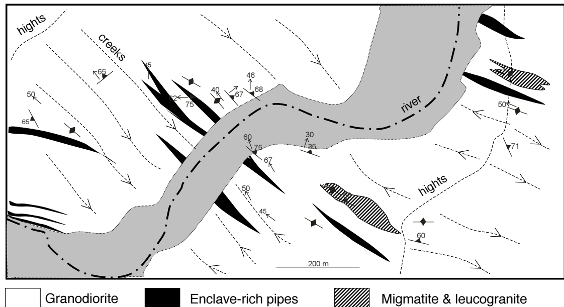
FIGURE 5 | Areal distribution and plan-view geometry of the subvertical, pipe-like structures of the Valle Fértil granodiorite. These are flatten pipes of few tens of meters width and extending for more than 200 m. Some are anastomosed and fish-shaped. They follow the magmatic foliations in the host granodiorite. Lineations, defined by the major axis of elongated enclaves are subvertical but dominantly dipping to the north.
