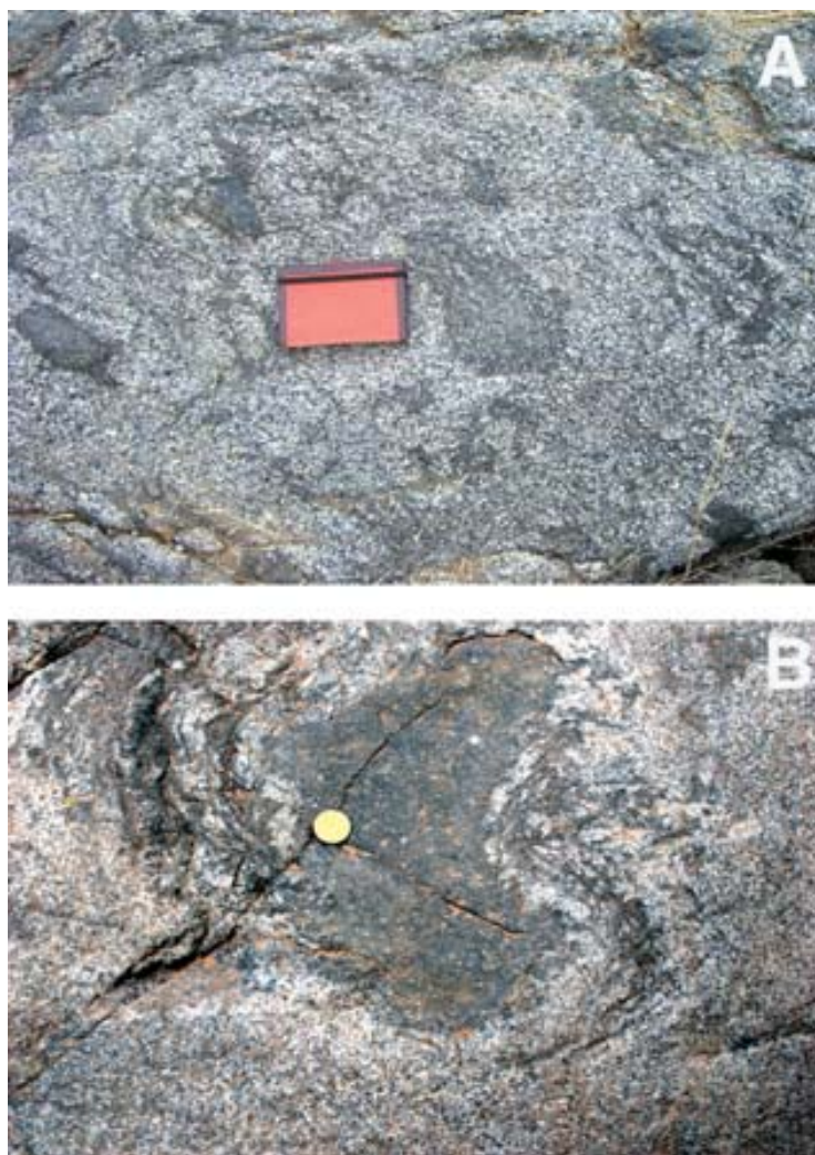
FIGURE 6 | Circular schlieren in horizontal sections within the pipe structures of Valle Fétil. A) Biotite-rich schlieren are around a microgranular enclave. B) Curved, near circular, schlieren and irregular enclaves. The same structures in the vertical section are strongly elongated defining a well marked magmatic lineation.
