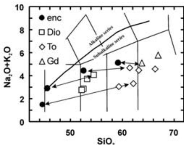
FIGURE 2 | Total alkalis versus \text{SiO}_2 diagram for the Valle Fertil granitoids and their enclosed microgranular enclaves. Granitoids display a typical subalkaline trend. Arrows connect the composition of each analyzed inclusion with its host granitoid.
