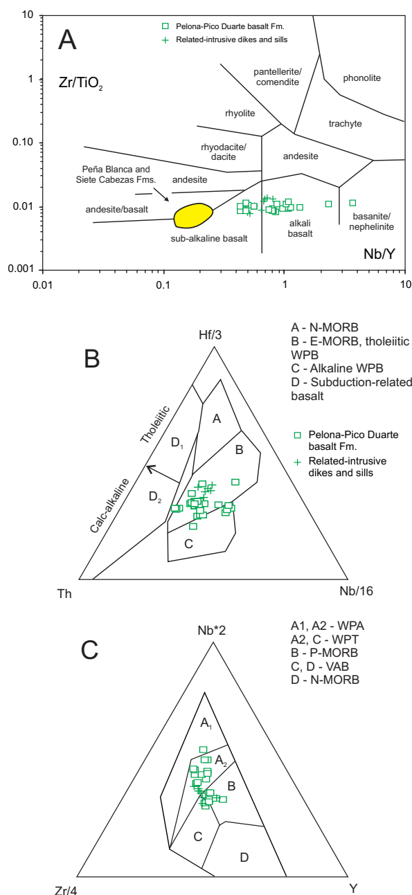
FIGURE 7 | A ) Nb/Y versus Zr/TiO 2 diagram of Winchester and Floyd (1977), for basalts, high-Mg basalts and related-intrusive dikes and of the PPDB in Central Hispaniola, B ) Hf-Nb-Th plot with fields defined by Wood (1980), and C ) Nb-Zr-Y plot with fields defined by Meschede (1986).
