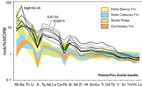
FIGURE 8 | MORB-normalized multi-element plots for the basalts of the Pelona-Pico Duarte Fm. The fields for geographically nearest CLIP units are shown for comparison (data taken from Révillon et al., 2000; Sen et al., 1988; Sinton et al., 1998; Escuder-Virue et al., 2008). Normalization values are taken from Sun and McDonough (1989).
