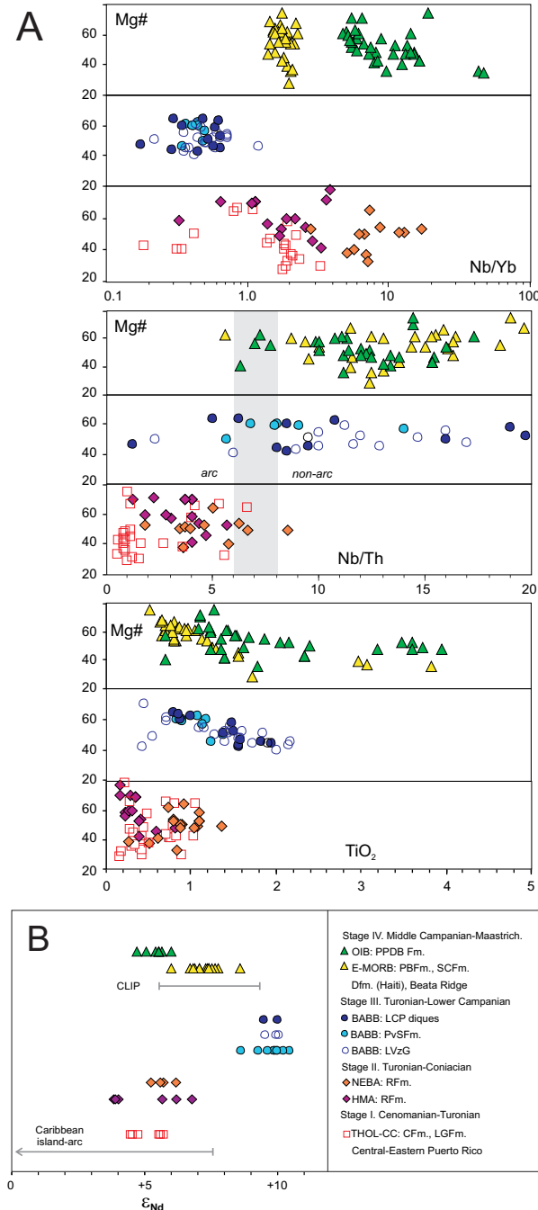
FIGURE 11 | A) Values of selected geochemical parameters and B) initial \epsilon_{Nd} values for the successive stages of the Late Cretaceous magmatic evolution of Central Hispaniola (Escuder-Virute et al., 2007, 2008, this work and unpublished). The Caribbean island-arc volcanic rocks of Puerto Rico are from Jolly et al. (2006, 2007, 2008). Beata Ridge data are from Révillon et al. (2000). THOL: tholeiitic; CC: calc-alkaline; RFm: Restauración Fm.; HMA: high-Mg andesites/basalts; NEBA: Nb-enriched basalts; BABB: back-arc basin basalts; CFm: Constanza Fm.; LGFm: Las Guayabas Fm. (Eastern Cordillera); LCP: Loma Caribe peridotite (Bonao block); LVZG: Los Velazquitos gabbros (Jarabacoa block); PVSFm: Peralvillo Sur Fm. (Bonao block); PBFm: Peña Blanca Fm.; SCFm: Siete Cabezas Fm. (NE sector Jarabacoa block); Dfm: Dumisseau Fm. (SW Haiti).
