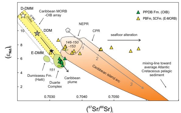
FIGURE 9 | Initial Sr-Nd isotopes ratios ( t=70\text{Ma} ) for the different Late Cretaceous basalts in Central Hispaniola. The fields for the Duarte Complex, DSDP site 15 (CLIP) and Caribbean island-arc lavas from Northeastern and Central Puerto Rico, are taken from Escuder-Virue et al. (2007a), Hastie et al. (2008; and references therein), Hauff et al. (2000), Jolly et al. (2006, 2007) and Thompson et al. (2004). The MORB-OIB array is defined by the subduction-unmodified lavas from the East Pacific Ridge (data from PETDB, 2007; and references herein). Depleted MORB mantle (DMM) Sr-Nd isotopic compositions are taken from Su and Langmuir (2003): DMM average for MORBs far from plumes; D-DMM is 2\sigma depleted and E-DMM is 2\sigma enriched over the average. Field and mantle components are age corrected. Caribbean island-arc field is subparallel to a calculated mixing line between pelagic sediments and representative arc basalt (Jolly et al., 2006; Escuder-Virue et al., 2008). NEPR: Northeastern Puerto Rico I-III (Albian-Maastrichtian); CPR: Central Puerto Rico I-IV (Albian-Maastrichtian).
