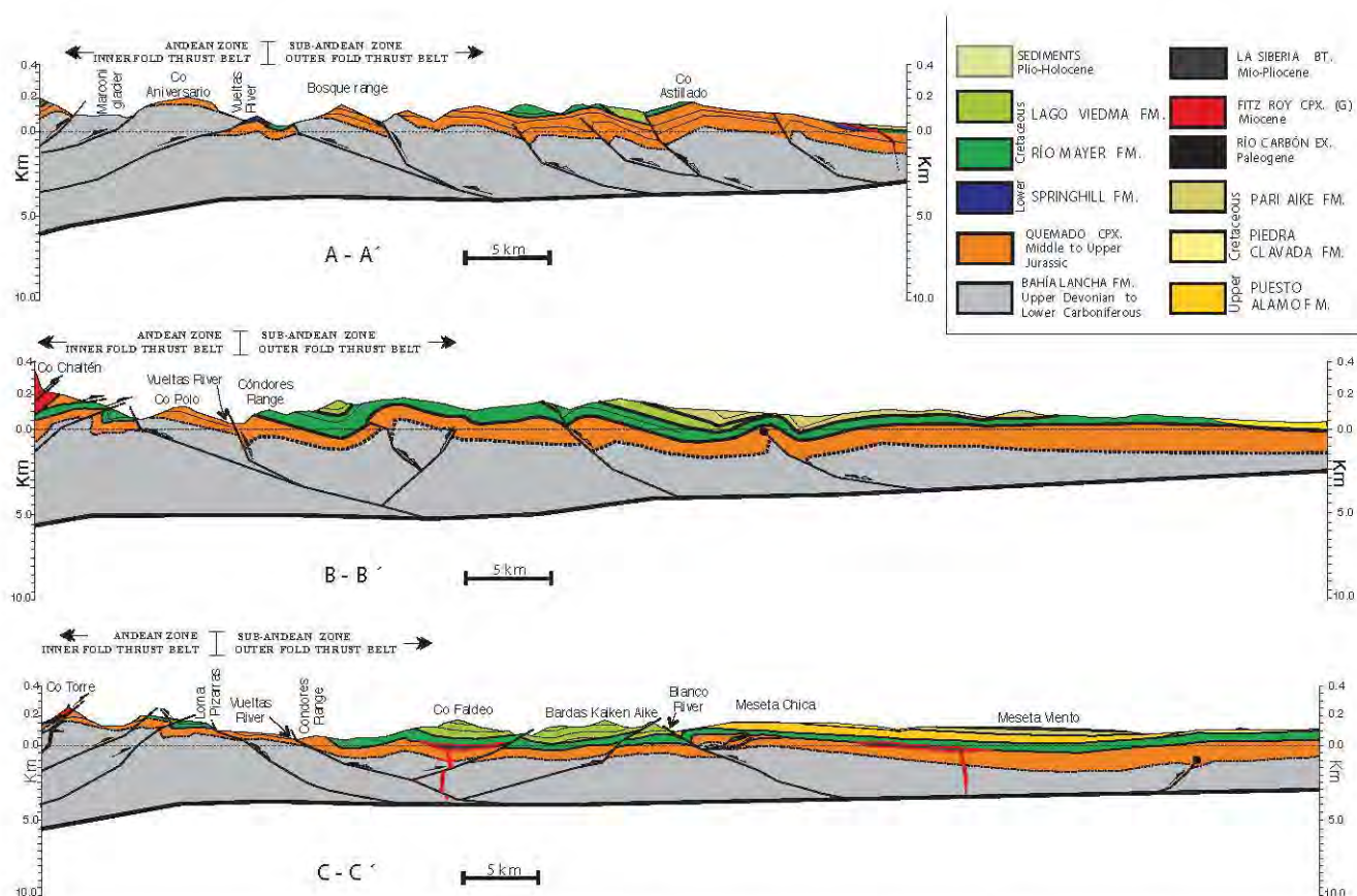
FIGURE 7 | Regional cross-sections (not balanced) between the San Martín and Viedma lakes. Seismic profile of Figure 9 is 10km south of section CC'. Location of sections lines is shown in Figure 4.
