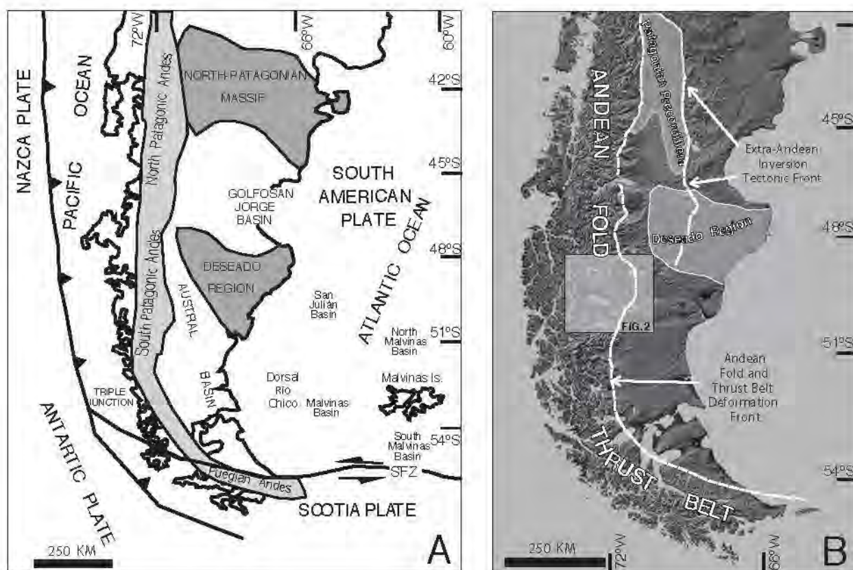
FIGURE 1 A) Major geological provinces and tectonic setting of Patagonia. B) Image showing the Andean fold thrust belt deformation front (Kraemer et al. , 2002), and the eastern boundary of the Tertiary inversion tectonic front in the Patagonian foreland (Giacosa et al. , 2010).
