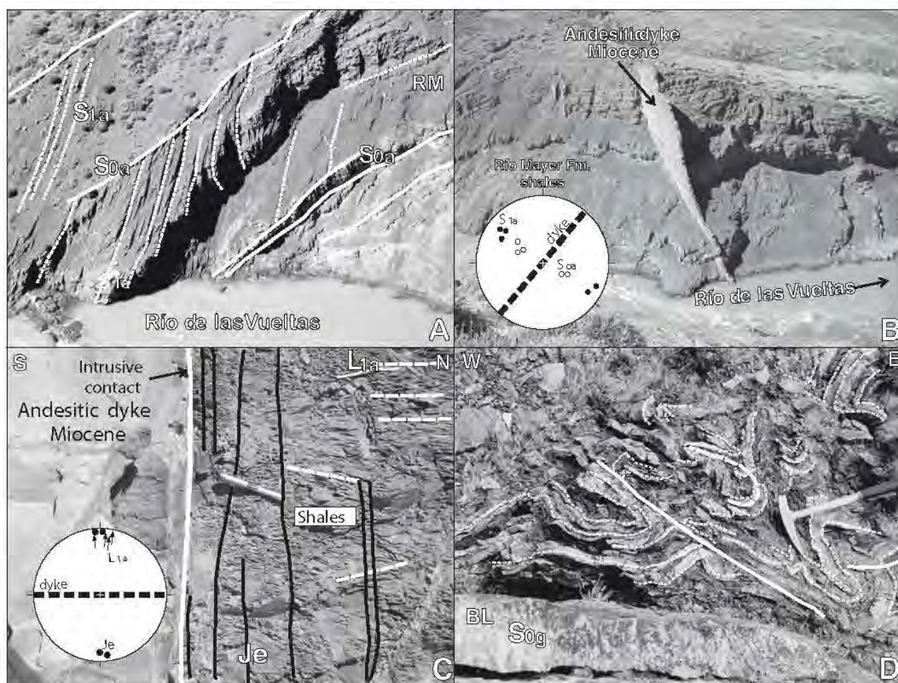
FIGURE 10 | A) The Río Mayer formation (RM) in the Vueltas river. Facies of black shales and laminated sandstones (bedding is S_{0a} ) with Andean axial planar cleavage ( S_{1a} ). B) Vertical andesitic dyke, to the Miocene magmatism (Fitz Roy plutonic complex), intruded deformed shales of the Río Mayer formation (RM). Stereonet shows the relations between dyke strike, bedding ( S_{0a} ) and axial plane cleavage ( S_{1a} ). C) The contact zone between andesitic dyke and shales of the Río Mayer formation in the Vueltas river. Andesitic dyke and cooling joints (Je) cutting the pencil lineation ( L_{1a} ) in the shales. Stereonet shows the relationships. D) Faulting and refolding in massive ortho-quartzites and pelites of the Bahía de la Lancha formation (BL) in the bridge over Eléctrico river. Refolding is near the fault plane in the hanging-wall of Bosques-Polo thrust. Thin dashed lines indicate bedding traces, solid lines faults and the thick dashed line show the approximate position of the refolded Gondwanan folds.
