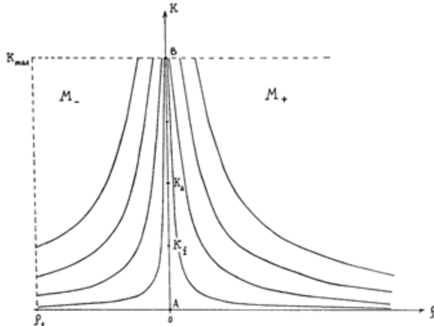
Fig. 1. Relation between the kinetic energy and mean spectral wave number of the R-H wave perturbations ( \alpha = 1 , K_{min} = 0 ).
