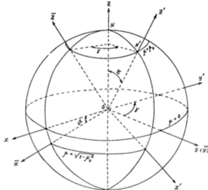
Fig. 2. The fixed coordinate system (x, y, z) and moving coordinate system (x', y', z') connected with the Rossby-Haurwitz wave (17) and modon (21) respectively. Coordinate system (\tilde{x}, \tilde{y}, \tilde{z}) demonstrates a position of system (x', y', z') at initial time.
