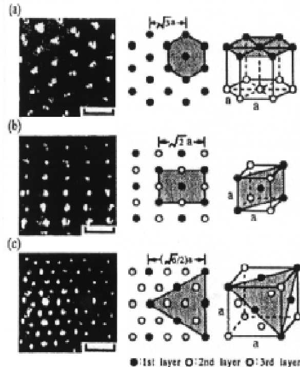
Fig. 8. Micrographs and sketches of the different crystal structures: (a) hexagonal; (b) bcc; (c) fcc. The center column corresponds to the structures in the micrographs. The graded areas in the sketches are normal to the optical axis. The bars correspond to 200\mu\text{m} .
