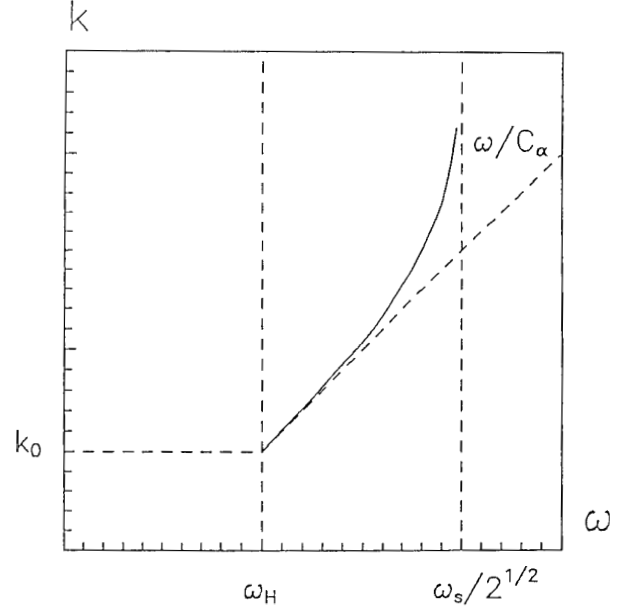
Fig. 4. Dependence k(\omega) for the surface wave in the case \vec{B}_0 \parallel \vec{k} .
