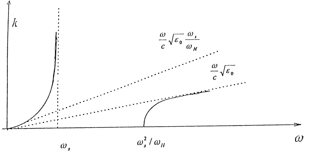
Fig. 2. Low-frequency electromagnetic waves for angle \theta = \pi/2 . In the frequency range 0 \leq \omega < \omega_s the wave is slow; in the frequency range \omega \geq \omega_s^2 / \omega_H the wave is fast.
