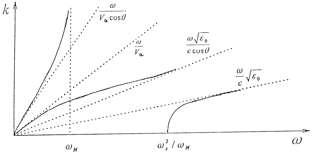
Fig. 3. Alfvén and magnetoacoustic waves.
