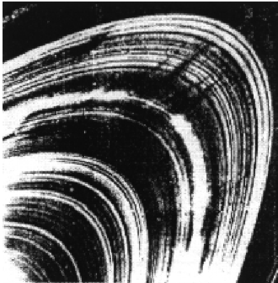
Fig. 6. The picture of the radial spokes in Saturn's ring. The azimuthal width of a spoke is typically a few thousand kilometers.
