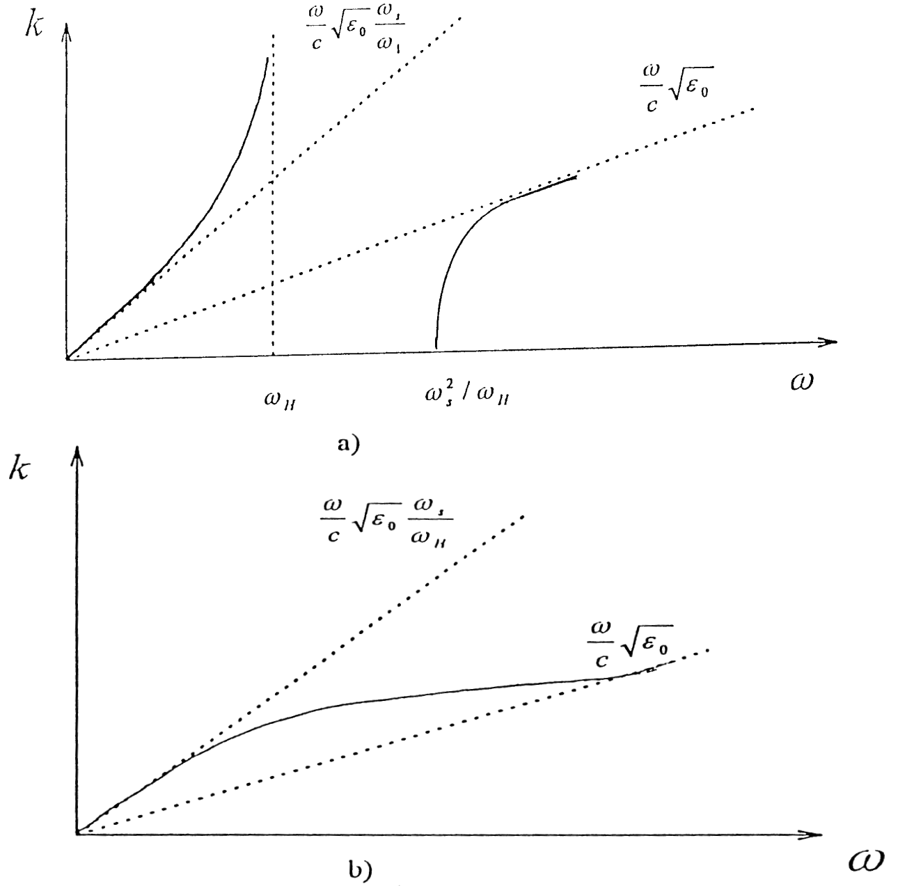
Fig. 1. Low frequency electromagnetic waves for the angle \theta = 0 . (a) Left-rotating: in frequency ranges 0 \leq \omega < \omega_H the wave is slow; in the frequency range \omega \geq \omega_s^2 / \omega_H the wave is fast; (b) right rotating: the wave exists in frequency range 0 < \omega < \infty .
