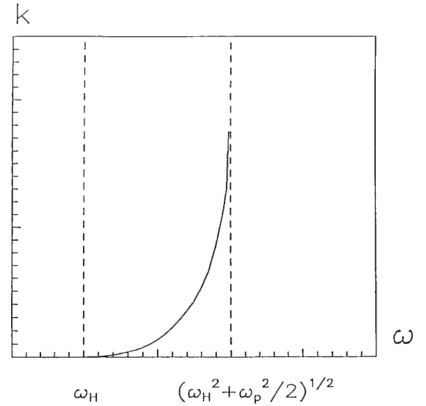
Fig. 5. Dependence k(\omega) for the surface wave in the case \vec{B}_0 \perp \vec{k} \perp \vec{N} .
