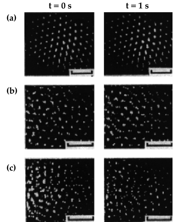
Fig. 7. Micrographs of hexagonal structures and more disordered structures at different power. The bars correspond to 500 \mu\text{m} .
