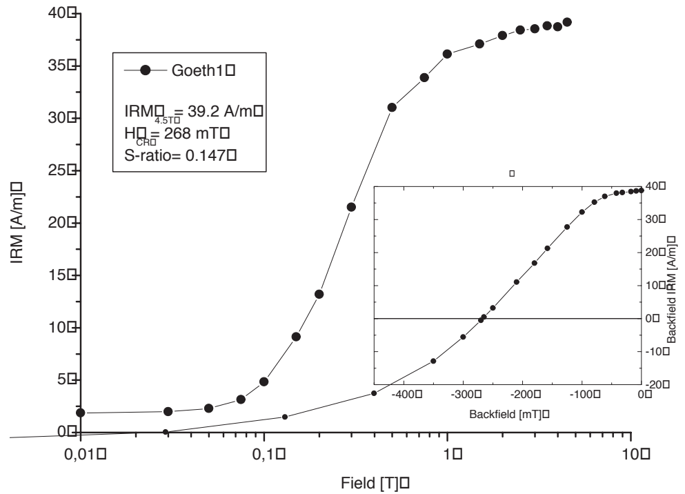
Fig. 3. IRM measurements. The highest applied field was 4.5 T. The following parameters were estimated: H_{CR} , S-ratio, S_{+40mT} y S_{+100mT} .
