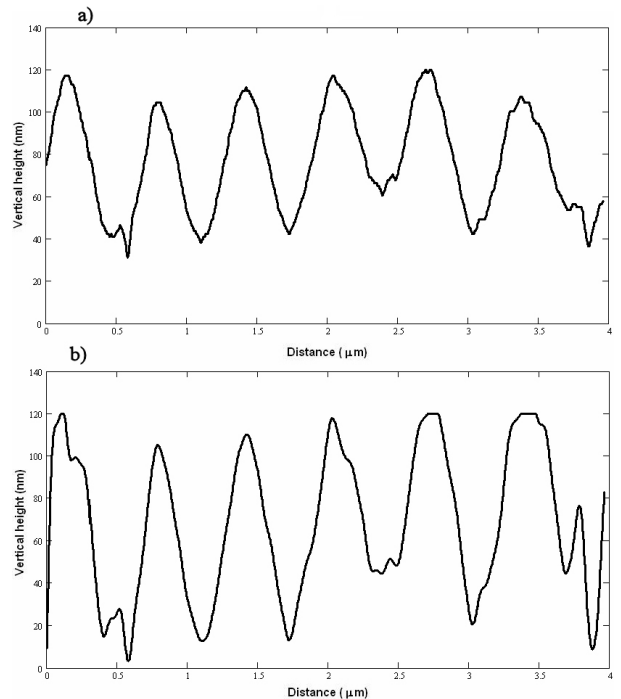
FIGURE 4. Line scans of a) DVD-R and b) DVD-R after the deconvolution process.
