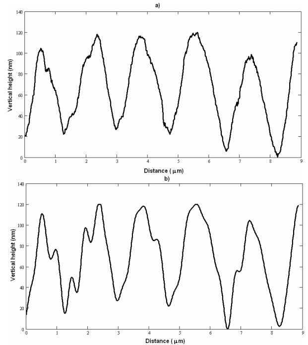
FIGURE 3. Line scans of a) CD-R and b) CD-R after the deconvolution process.
