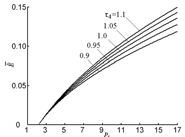
FIGURE 3. Effect of the ratio of hot-side heat reservoir inlet temperature to ambient temperature on the dimensionless ecological function vs. pressure ratio.
