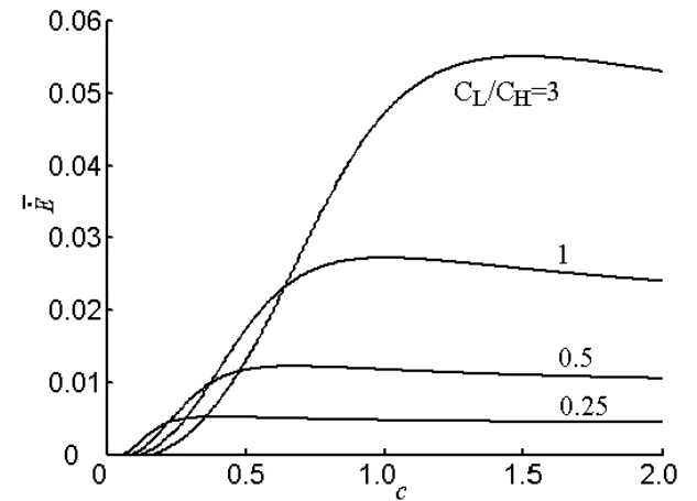
FIGURE 9. Effect of the ratio of heat reservoirs capacitance rate on the dimensionless ecological function vs. heat capacity rate matching between the working fluid and heat reservoirs.
