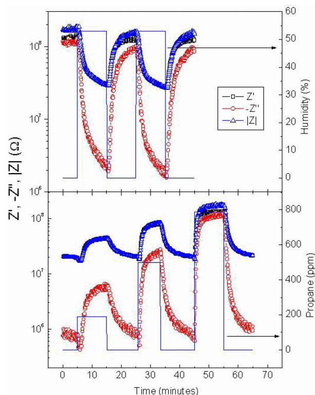
FIGURE 6. Dynamical responses of the hematite film (2% Zn) at 30 °C measured with a 100 Hz, 30 mV sinusoidal voltage. In the upper graph the response of the total impedance and its real and negative imaginary parts are depicted, along with the humidity profile applied. The lower graph depicts the similar responses to different concentrations of propane as indicated by the continuous line, added to humid air.
