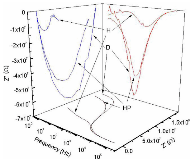
FIGURE 4. Projections of the three-dimensional paths defined by Z'' vs. both, Z' and the measurement frequency, according to Macdonald et al. In this case, results for the sample with 2% Zn at 30^\circ\text{C} are shown. In each coordinate plane, three projections are plotted: one for the dry air response (D), the second for the humid air atmosphere (H) and the third one for the humid air plus propane (HP) response. As projections on the coordinate planes, the real and imaginary parts of the impedance are shown as a function of frequency in the horizontal and right-side vertical planes. Besides, the imaginary vs. the real part is also plotted in the left-side vertical plane.
