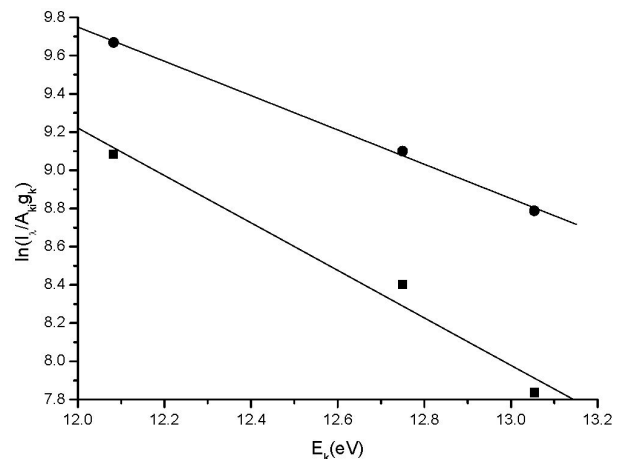
FIGURE 3. Boltzmann plot for \alpha , \beta and \gamma hydrogen lines at (●) 532 nm and (■) 1064 nm.
