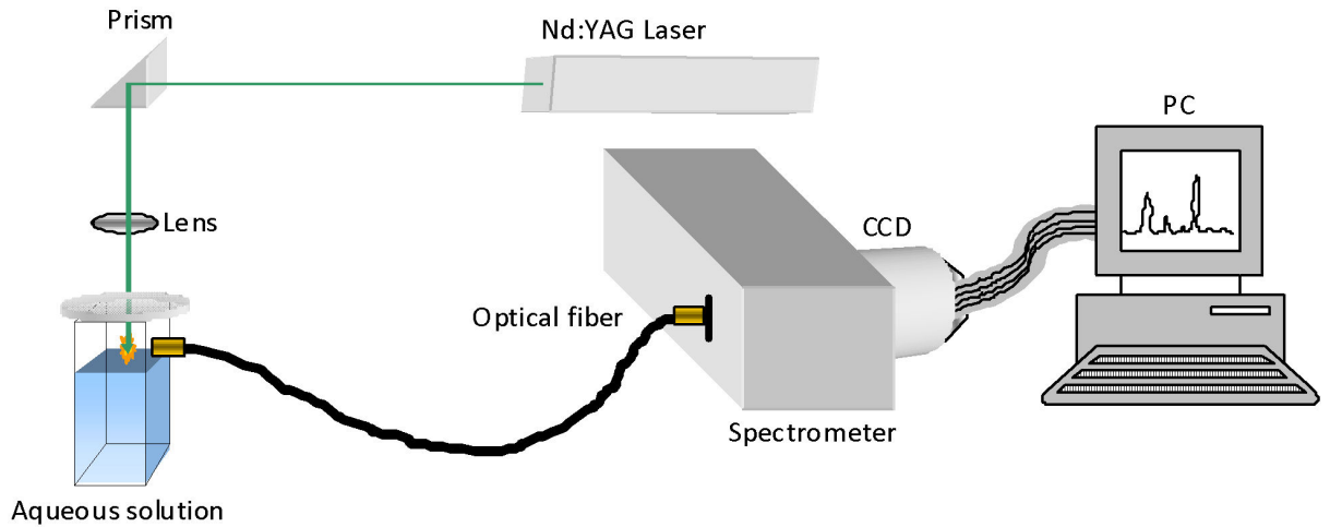
FIGURE 1. Experimental setup.
