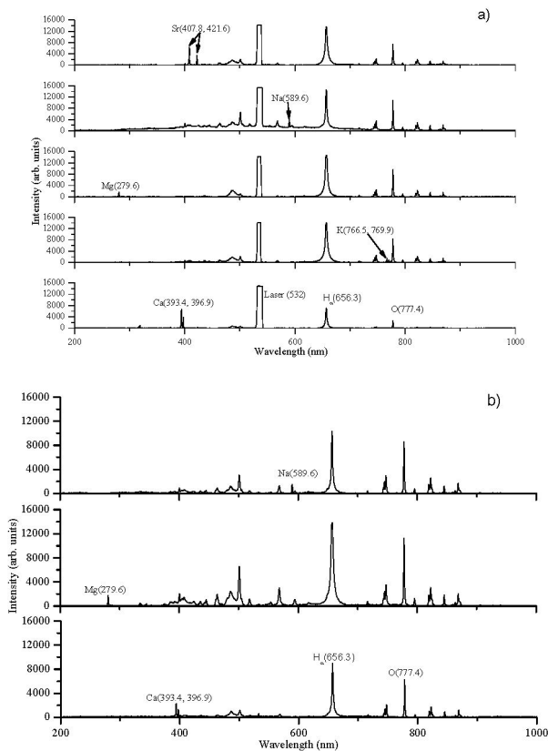
FIGURE 2. LIBS spectra of Ca, K, Mg, Na and Sr aqueous solution at (a) 532 nm and (b) 1064 nm
