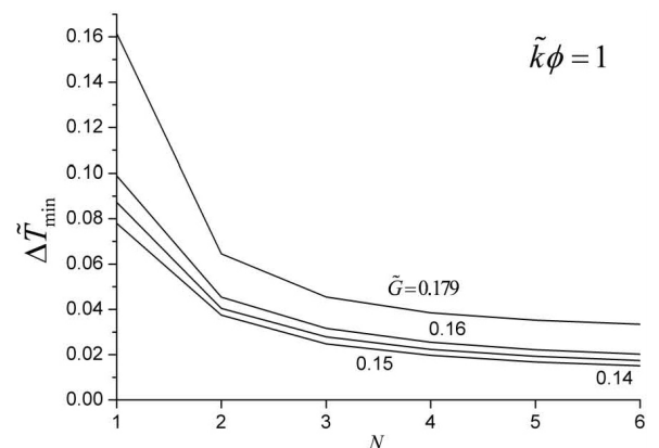
FIGURE 3. Effect of \tilde{G} on \Delta \tilde{T}_{min} versus N with fixed \tilde{k}\phi .
