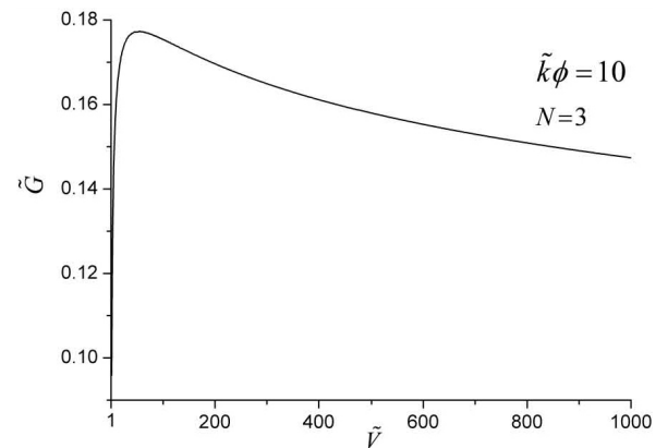
FIGURE 11. \tilde{G} corresponding to (\tilde{G}/\Delta\tilde{T})_{\max} versus \tilde{V} .
