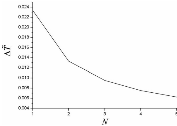
FIGURE 7. \Delta\tilde{T} corresponding to (\tilde{G}/\Delta\tilde{T})_{\max} versus N .
