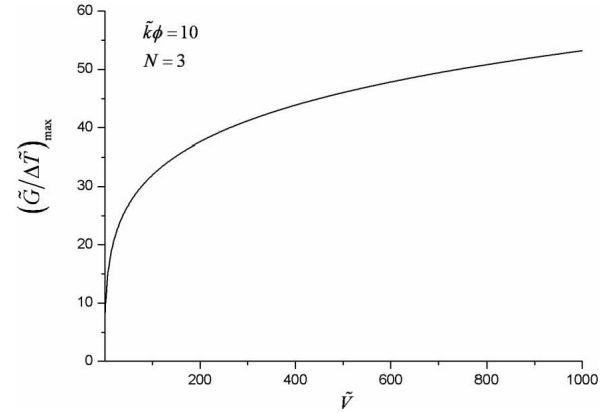
FIGURE 9. (\tilde{G}/\Delta\tilde{T})_{\max} versus \tilde{V} with fixed \tilde{k}\phi and N .
