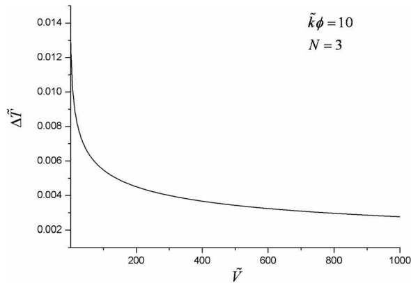
FIGURE 12. \Delta\tilde{T} corresponding to (\tilde{G}/\Delta\tilde{T})_{\max} versus \tilde{V} [33].
