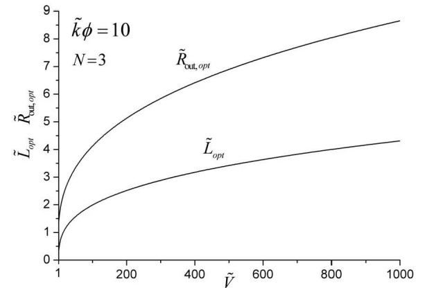
FIGURE 10. Optimal geometries (\tilde{L}_{opt}, \tilde{R}_{out,opt}) corresponding to (\tilde{G}/\Delta\tilde{T})_{\max} versus \tilde{V} .
