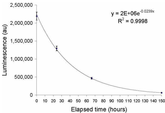
FIGURE 4. OSL fading curve of the optical fiber.
