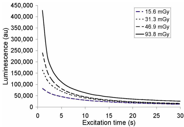
FIGURE 2. CW-OSL curves for four different gamma radiation doses.
