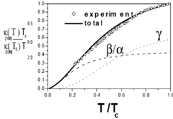
FIGURE 2. Numerical fit of the in-plane thermal conductivity components [100] normalized at T_c . Experimental data is taken from [10].
