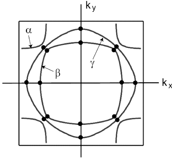
FIGURE 1. The black dots show the positions of the point nodes in the superconducting gap on the \beta and \gamma Fermi surface sheets in \text{Sr}_2\text{RuO}_4 , as determined by Eqs. 2 and 3. Each solid circle represents two nodes, at positions \pm k_z .
