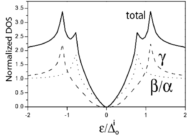
FIGURE 3. Numerical calculations of the superconducting density of states DOS for the \beta and \gamma sheets according to our model.
