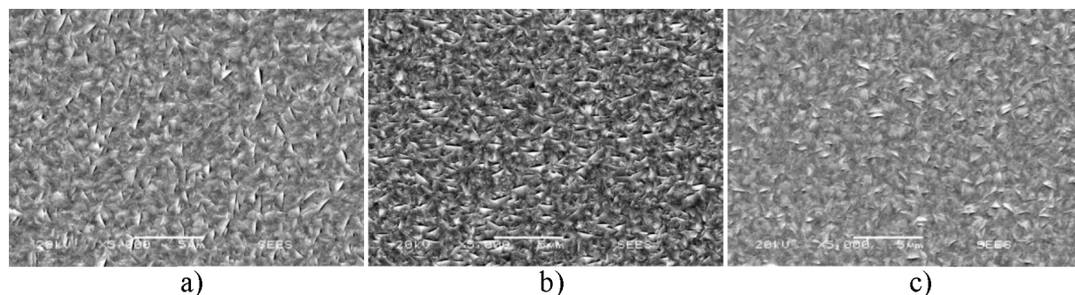
FIGURE 2. Surface SEM images of a) CIGS-8C, b) CIGS-12, and c) CIGS-13 samples.
