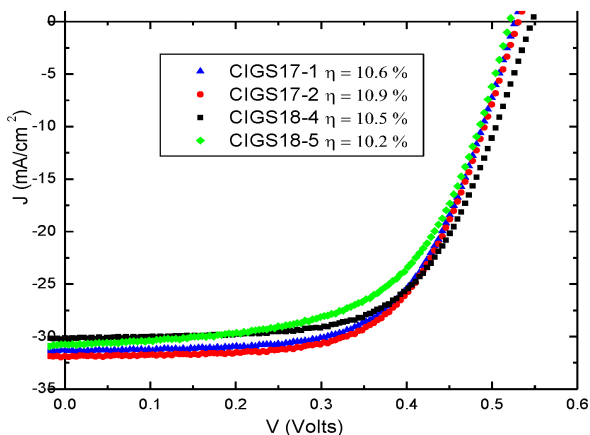
FIGURE 6. J-V characteristics of CIGS thin film solar cells under AM1.5 illumination. They were measured at 25°C on an effective area of 0.47 cm 2 .
