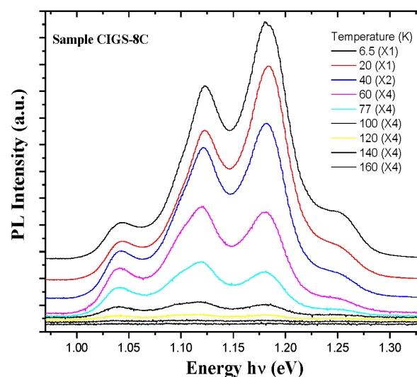
FIGURE 4. PL spectra as a function of temperature for co-evaporated CIGS-8C thin film.
