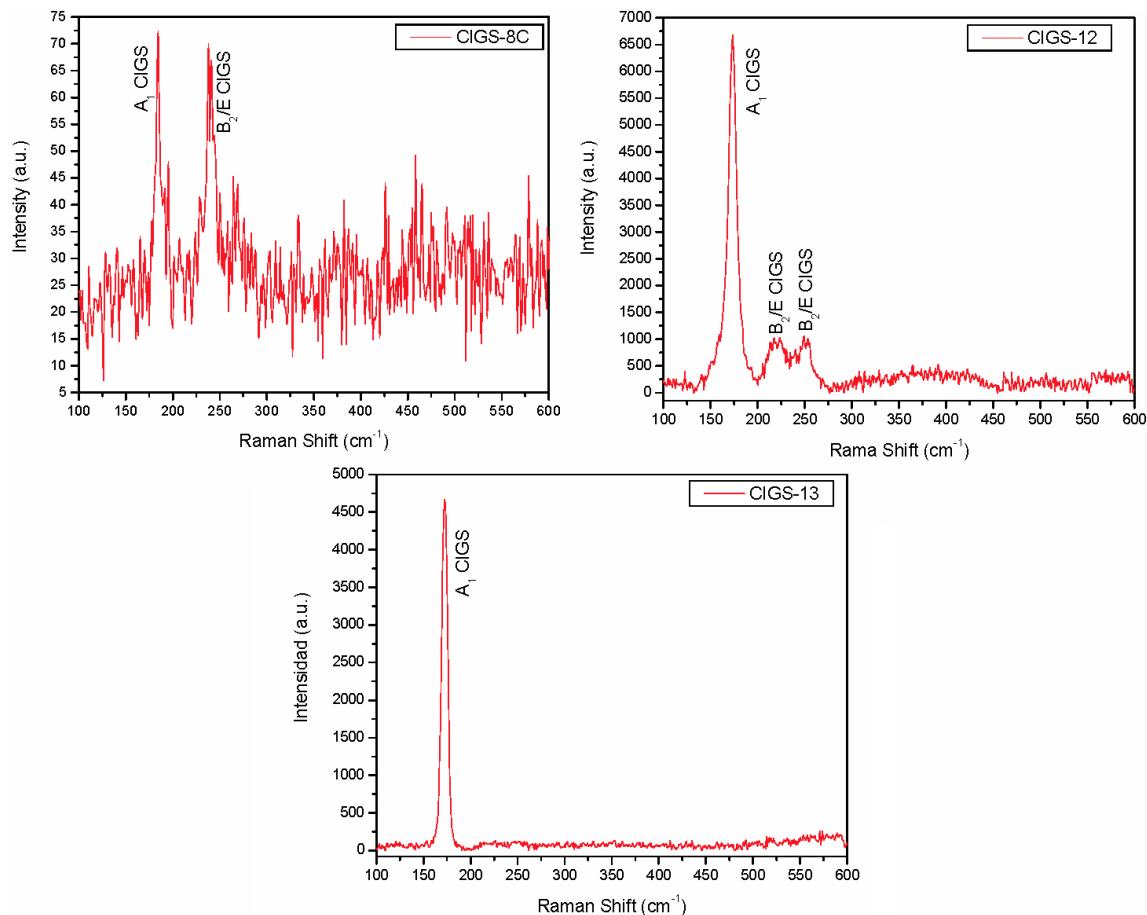
FIGURE 5. Raman spectra of CIGS thin films grown on glass/Mo substrate by co-evaporation.
