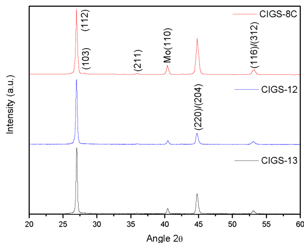
FIGURE 3. XRD patterns for CIGS-8C, CIGS-12 and CIGS-13 samples prepared by co-evaporation.
