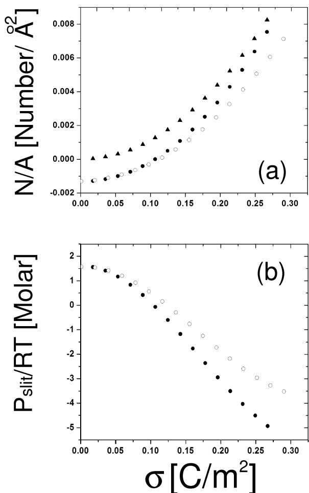
FIGURE 1. (a) calculated excess of counterions N/A as a function of surface charge density \sigma . Predictions using liquid theory; symbol \circ for discrete, and \bullet smooth surface charge respectively, and mean field result \blacktriangle for case of smooth surface charge only. System; restricted primitive model of 1:1 electrolyte at 1 M concentration between two infinite flat walls separated 9 Å. Figure (b) are the liquid theory predictions of slit pressure P_{\text{slit}}/RT versus surface charge density \sigma for \circ discrete, and \bullet smooth surface charge, respectively.
