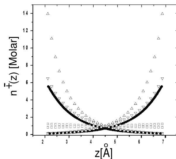
FIGURE 2. Calculated profile concentrations of ions between the two walls with smooth surface charge; mean field results are the symbols \triangle , \nabla , \square , for \sigma = 0.256, 0.178, 0.0178 C/m 2 , respectively. AHNC result corresponds to \bullet symbol with \sigma = 0.16019 C/m 2 . Other system parameters as in Fig. 1.
