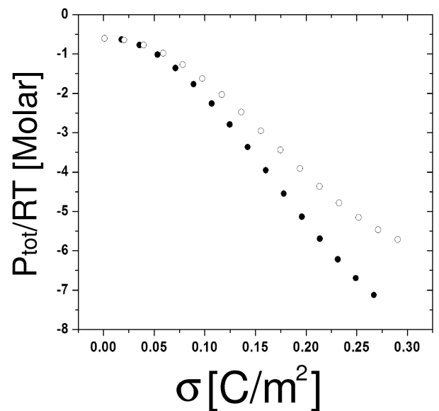
FIGURE 4. AHNC prediction of total pressure between the two walls for discrete \circ , and smooth \bullet density of surface charge \sigma . Same system parameters as in Fig. 1, and \phi = 1.094 .
