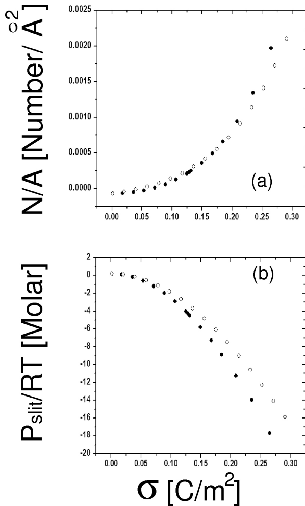
FIGURE 3. Liquid theory prediction of excess of counterions (a) and slit pressure (b) as a function of surface charge for discrete \circ , and smooth \bullet density of surface charge. Wall's separation is 9 Å and salt concentration 0.1 M.
