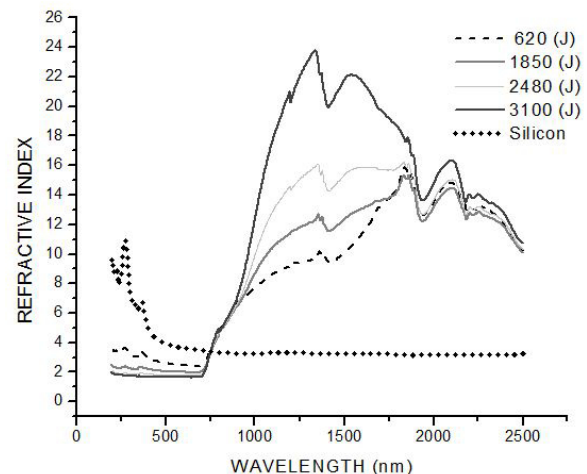
FIGURE 6. Calculated refractive index of untreated silicon and of silicon irradiated with gas assistance.
