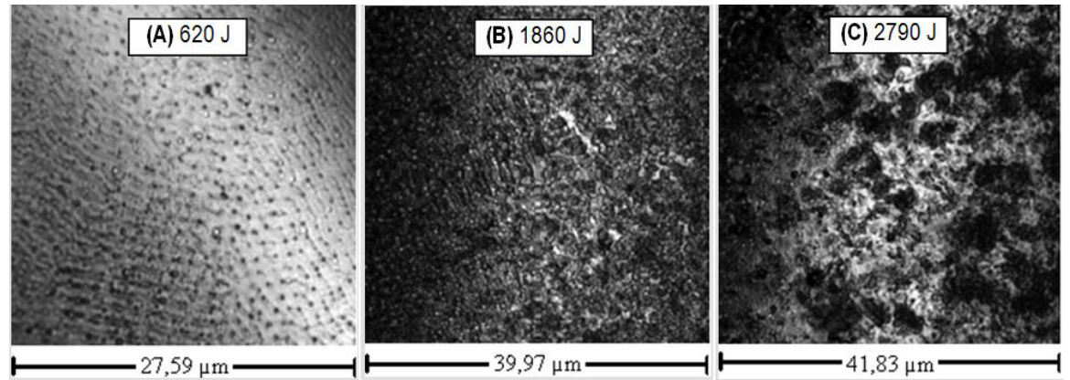
FIGURE 7. Confocal microscope images of samples irradiated without argon gas blowing. Each image is labeled with the energy applied.
