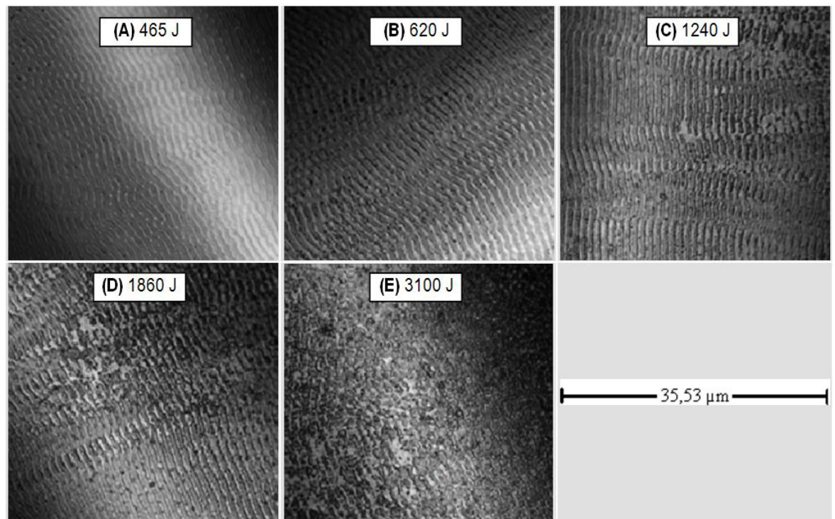
FIGURE 2. Confocal microscope images of samples irradiated with different amounts of energy and argon gas blowing.
