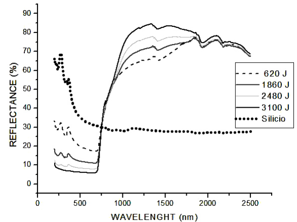
FIGURE 5. Results of diffuse reflectance tests on laser irradiated and on untreated silicon samples.
