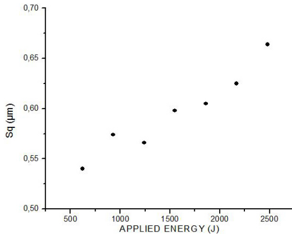
FIGURE 4. Root mean square height ( S_q ) of the periodic structures as a function of the applied energy.
