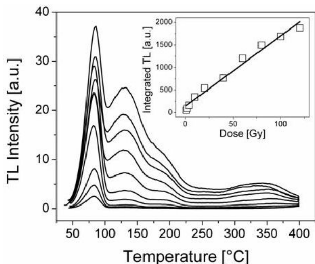
FIGURE 2. TL glow curves of the polyminerals expose to different doses, namely 120, 100, 80, 60, 40, 20, 10, 4, 2 and 1 Gy, from top to bottom. In the inset: integrated TL response as a function of the gamma doses (1-120 Gy).
