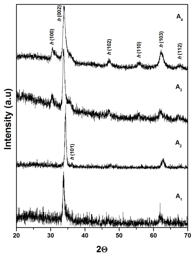
FIGURE 1. X-ray diffraction patterns of ZnO and ZnO:Al films deposited at RT by RF co-sputtering from a ZnO-Al target. The meaning of h on the plane indexes is hexagonal.
