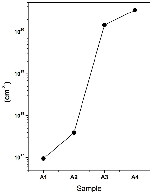
FIGURE 5. Carrier concentration of ZnO and ZnO:Al films studied in this work.
