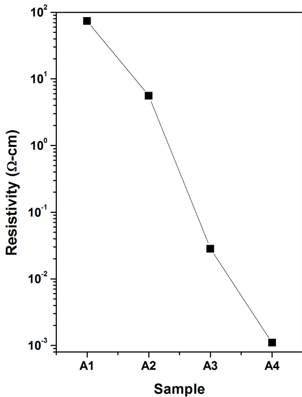
FIGURE 4. Resistivity of ZnO and ZnO:Al films grown by RF sputtering on glass substrates.
