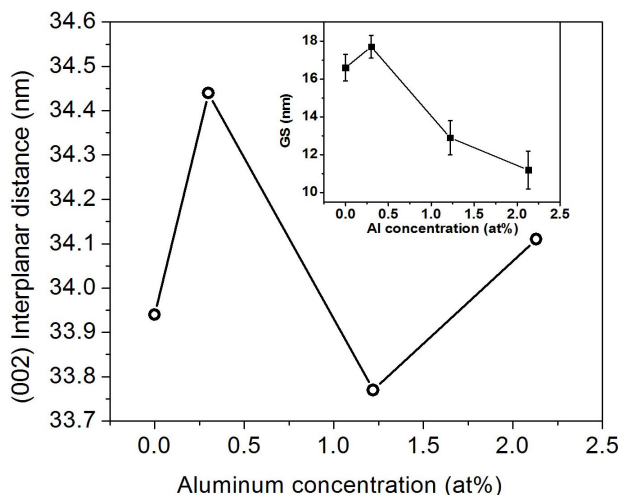
FIGURE 2. The (002) interplanar distance versus the Aluminum concentration. The inset illustrates the grain size as a function of the Al concentration.
