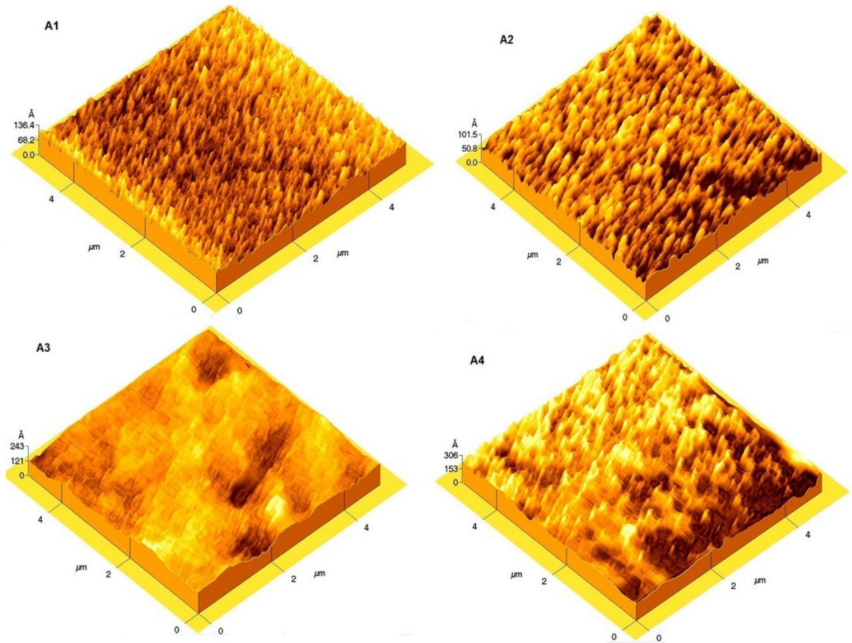
FIGURE 3. 3D AFM images of ZnO and ZnO:Al samples prepared at RT. The image scale is 5 \times 5 \mu\text{m} .
