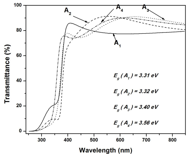
FIGURE 6. Transmission spectra of A1-A4 films. Energy gaps of the films are also displayed.
