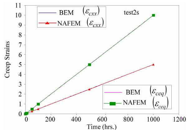
FIGURE 6. Creep strain distribution for a biaxial load in secondary creep analysis.
