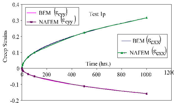
FIGURE 2. Creep strains for uniaxial load in a primary creep analysis.
