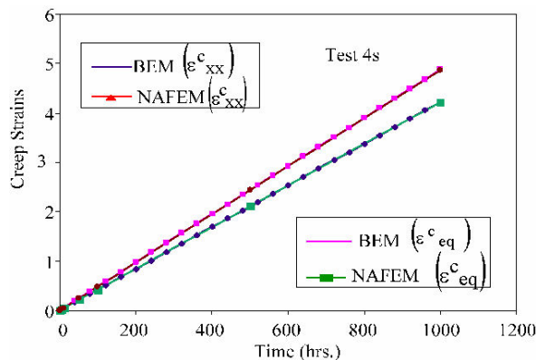
FIGURE 8. Creep strain distribution in a biaxial load.
