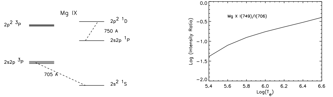
Fig. 3. ( Left ) Schematic energy level diagram for the Be-like ion Mg IX. ( Right ) Intensity ratio of the 2p^2\ ^1D_0 - 2s2p\ ^1P_1 line to the 2s2p\ ^3P_1 - 2s^2\ ^1S_0 as a function of temperature.
