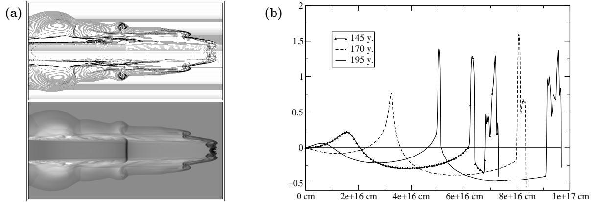
Fig. 1. (a) Poloidal magnetic field lines (top frame) and the logarithm of the density (bottom frame) where black (white) is high (low). (b) Scaled logarithm of the toroidal field strength along the jet beam at 3 times.
