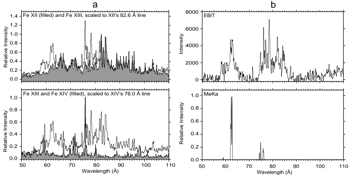
Fig. 2. (a) Mixed Fe XIII compared with spectra of lower (top) and higher (bottom) beam energies. (b) Pure Fe XIII from EBIT compared calculations from the MeKa database (Kaastra & Mewe 1993).
