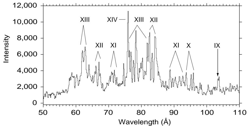
Fig. 1. Spectrum at beam energy of 330 eV. Fe XIII is dominant, but Fe IX – Fe XIV are also present.
