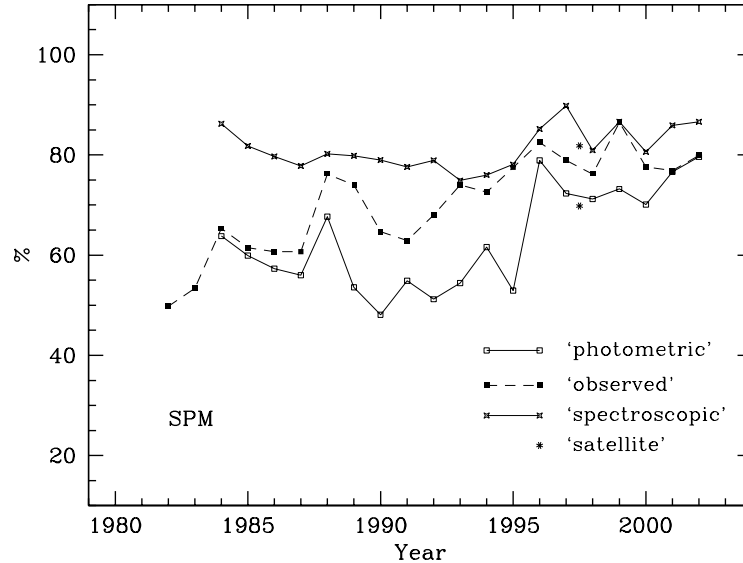
Fig. 2. Yearly fraction of nights of photometric and spectroscopic quality in San Pedro Mártir during the period January 1984 - December 2002. Also shown is the actual use of the 2.1m telescope from July 1982 to December 2002. The asterisks refer to the mean satellite June 1997 - May 1998 measurements by Erasmus and van Staden (2002).
