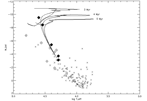
Fig. 4. Preliminary H-R diagram of IC 1795. Solid points show stars having spectroscopic classifications; open squares show stars placed on the basis of high quality photometric data; and crosses show the remainder of the stars observed. Isochrones for 3, 4, and 5 Myr from Schaller et al. (1992) are overlaid.
