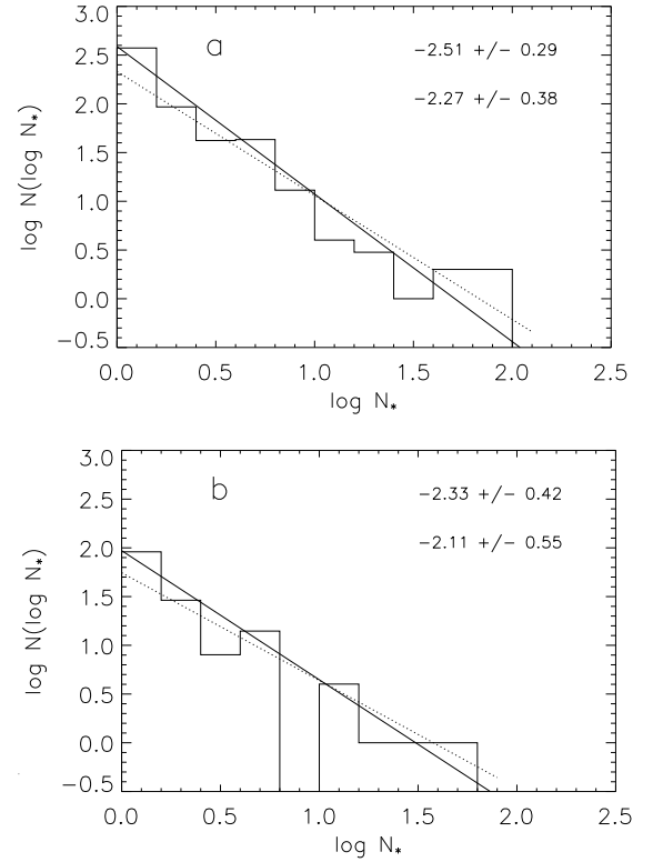
Fig. 1. Clustering relations for the candidate (a) OB sample and (b) O-star sample. The solid and dotted lines show power-law fits for the entire distribution and omitting the field stars, respectively.
