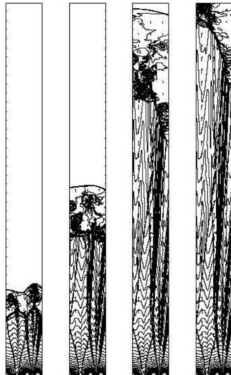
Fig. 4. The multiple winds density distribution. The evolutionary time in the panels is 1.62 \times 10^5 yr, 4.17 \times 10^5 yr, 9.4 \times 10^5 yr and 1.25 \times 10^6 yr, respectively.
