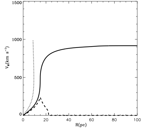
Fig. 1. Three possible types of integral curves. 1) The stationary wind solution (solid line), R_{sonic} = R_{sc} . 2) The breeze solution (dashed line), R_{sonic} > R_{sc} . 3) Unphysical double valued solution (dotted line), R_{sonic} < R_{sc} . For the three examples we adopted \dot{E}_{sc} = 10^{41} erg s^{-1} , R_{sc} = 15 pc, V_{\infty A} = (2q_e/q_m)^{1/2} = 1000 km s^{-1} .
