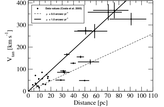
Fig. 1. Derived tangential velocities vs. distance for the sample objects in Costa et al. (2005). Distance error bars have been computed from the derived parallax errors. It is clear that our 2-4 mas error budget limits the usefulness of these parallaxes to objects closer than about 30 pc. We can also clearly see the kinematic bias introduced in the input sample by the high proper motion selection criteria: The solid and dashed line indicate a fixed proper motion of 1.0 and 0.5 arcsec yr -1 , respectively.
