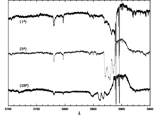
Fig. 3. The evolution of Na I D absorption in Nova Ophiuchi 2004. Note the progressive blueward migration of the stronger doublet components—a sign of outwardly accelerating gas.
