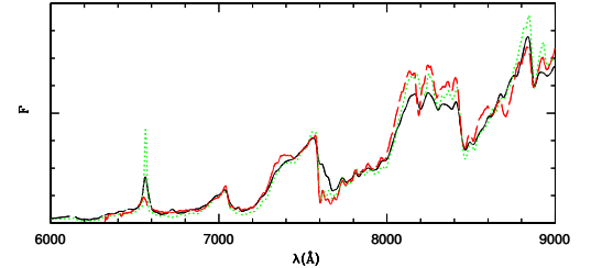
Fig. 1. Spectra of an M8 SFR member (solid), superimposed with library spectra of a young M8 dwarf (dotted) and an M8 field star (dashed). All spectra were normalized and shows that the NaI (8200 \text{\AA} ) absorption feature of the candidate, corresponds to a low surface gravity young object.
