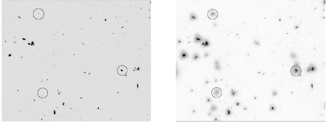
Fig. 2. Small piece (0.3%) of GOODS field showing three X-ray sources ( circles ). Left : HST multicolor image. The X-ray source on the right is unabsorbed, according to its X-ray spectrum, and indeed is bright in the optical. The two X-ray sources on the left are heavily absorbed, and very faint and red in the optical. Right : HST image with Spitzer 3.6-micron image superimposed. Both optically-faint AGN are bright in the infrared, as expected if the absorbed UV/X-ray light is reradiated by dust.
