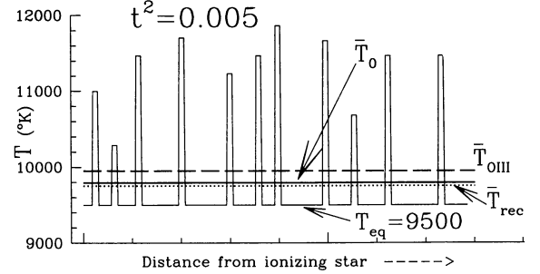
Fig. 1. A numerical simulation of temperature fluctuations consisting of hot spots characterized by an amplitude t^2 = 0.005 (from eq. 2). The mean temperature \bar{T}_0 obtained from applying eq. 1 is 9800 K (horizontal solid line). Also shown the relative position of \bar{T}_{rec} and T_{[O III]4363} . The fluctuations' lower bound temperature (to be associated to T_{eq} ) is 9500 K.
