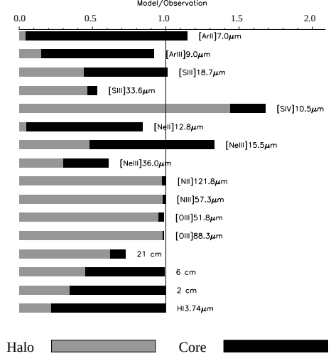
Fig. 1. Ratios of the modeled to observed line intensities and radio continuum flux densities. The line intensities are taken from Peeters et al. (2001).
