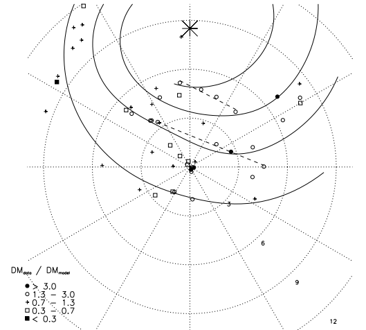
Fig. 2. DM_{\text{data}}/DM_{\text{model}} for pulsars with |z| < 300 pc. The grid circles are labeled with distance from the Sun, and the star marks the center of the galaxy. Notice lines of high DM_{\text{data}} at \approx 2 and 5 kpc towards the Galactic center, with regions of fair fit between. The first line coincides with the location of one of the Galactic arms (shown) of the Taylor & Cordes (1993) model.
