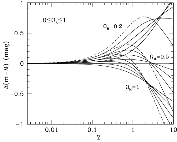
Fig. 1. Normalized distance modulus \Delta(m - M) = (m - M)_{\Omega_M, \Omega_\Lambda} - (m - M)_{.5, 0} as a function of redshift. For each value of \Omega_M as labeled in the Figure we plot a family of vacuum energy density \Omega_\Lambda = 0, 0.25, 0.5, 0.75, 1.0 . For each family, the dashed line corresponds to \Omega_\Lambda = 1 .
