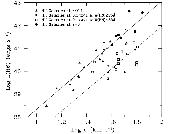
Fig. 2. The Luminosity- \sigma correlation for H II galaxies at a wide range of redshifts. The solid line shows the Maximum-Likelihood fit to the young H II galaxies in the local Universe. The dashed line shows the predicted L(H\beta) - \sigma relation for an evolved population of H II galaxies. The cosmology is H_0 = 65 , q_0 = 0 , \Lambda = 0 .
