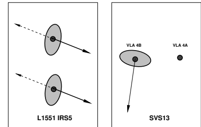
Fig. 3. Cartoon illustrating two possible scenarios in the formation of a binary system. In the L 1551-IRS 5 scenario (left) both protostars develop a disk-jet system, while in the SVS 13 scenario (right) only one protostar develops a disk-jet system.
