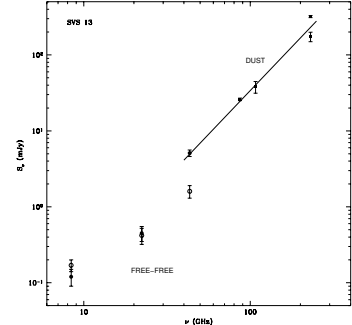
Fig. 2. Spectrum of SVS 13 from 3.6 cm to 1.3 mm. Open circles correspond to the emission of VLA 4A, while filled circles correspond to the emission of VLA 4B. The solid line is the best linear fit to the overall dust emission from 3.4 to 1.3 mm (filled squares). Note that the measured flux density of VLA 4B at 7 mm fits very well on the extrapolation of the millimeter dust emission, while the 7 mm flux density of VLA 4A appears to correspond to free-free emission, which dominates in the centimeter range. Adapted from Anglada et al. (2003a).
