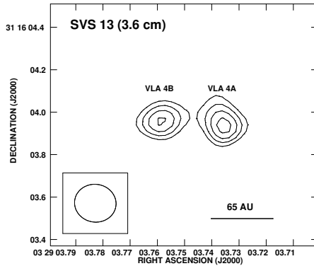
Fig. 1. VLA map at 3.6 cm of SVS 13, revealing that it is a binary radio source. Contour levels are -3 , 3 , 4 , 5 , and 6 times 14 \mu\text{Jy beam}^{-1} . The half power contour of the synthesized beam is shown in the lower left corner. Adapted from Anglada et al. (2000).
