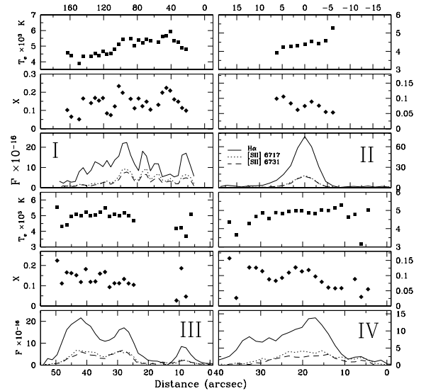
Fig. 1. Spatial distribution of the derived electronic temperature ( T_e ) and ionization fraction ( X ) along slits I, II, III and IV. We show the spatial intensity distribution of H \alpha and [S II] 6717/31 lines.
