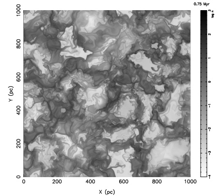
Fig. 1. The first star, having a mass of 20 M_{\odot} , explodes at x = 220 , y = 400 pc, defining the origin of the LB.
