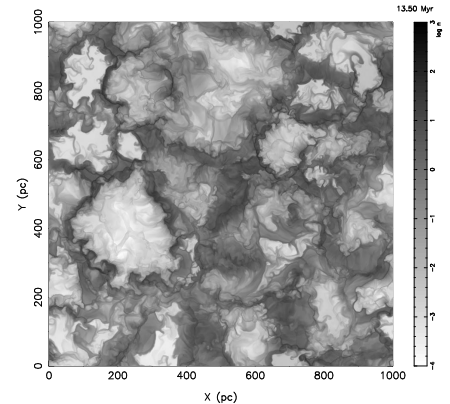
Fig. 2. The local bubble at time 13.50 Myr after the 20th supernova, which originated from a 10 M_{\odot} star, occurred.
