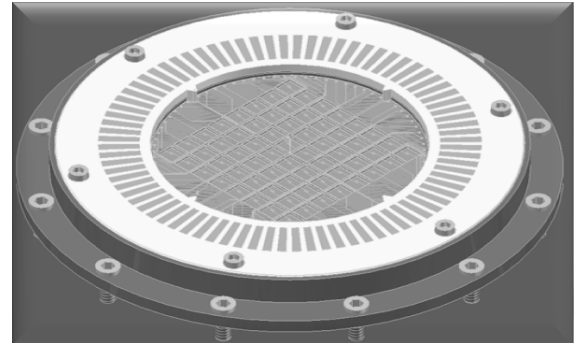
Fig. 7. 3D model for 8 × 8 elements bolometer, Copper base and Teflon ® printed circuit board for electrical connections.
