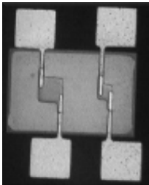
Fig. 1. Picture of two bolometers over a Silicon Nitride diaphragm developed at INAOE (Heredia 2004).
