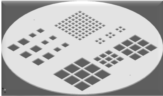
Fig. 2. 3D model for wafer micromachining structure.
