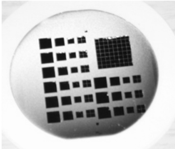
Fig. 5. Picture of 45° rotate masks wafer experimental micromachining results.
