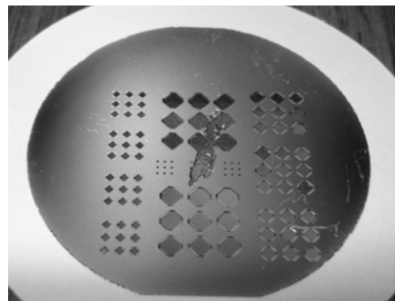
Fig. 4. Picture of 45° rotate masks wafer experimental micromachining results. All diaphragm support their own weight.
