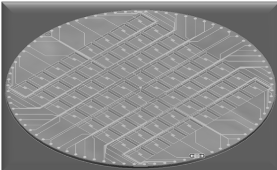
Fig. 6. 3D model for final 8 × 8 elements bolometer array of 3mm × 3mm.
