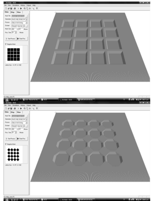
Fig. 3. 4 × 4 elements micro machined array simulation made with ACES with (110) planes parallel to masks (up) and rotated 45° respect same plane (bottom).
