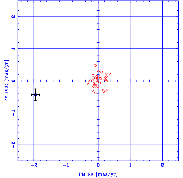
Fig. 1. Vector point diagram of the LMC QSO field described here.
