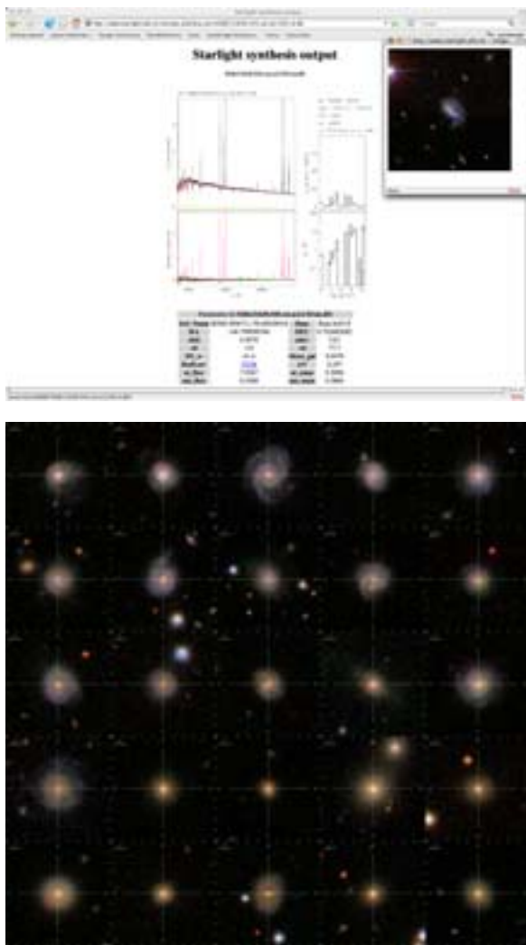
Fig. 1. Top : Screen-shot showing an example database query. Bottom : Galaxies of same stellar mass ( 10^{11.00 \pm 0.05} M_{\odot} ) and redshift ( 0.07 \pm 0.01 ), low inclination ( b/a \geq 0.9 ) sorted according to the STARLIGHT-derived (light-weighted) mean stellar age: \log t [yr] = 8.3 to 10.3, increasing to the right and from the top. Color plots are available in the electronic version of this paper.
